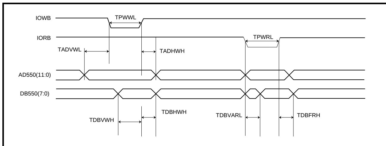
FIGURE 10: AC Timing
