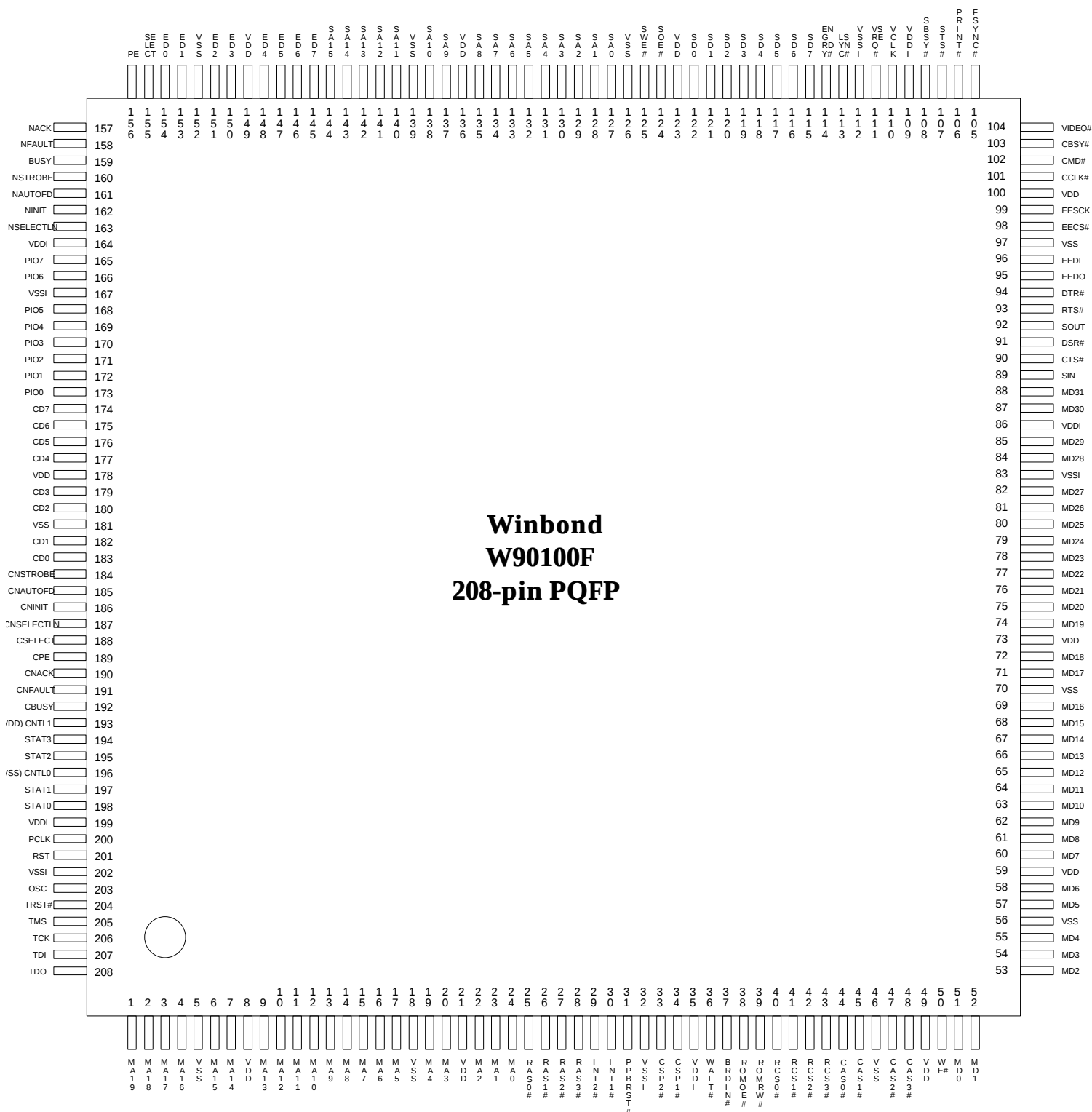
Figure 3.1 W90100 Pin Configuration
