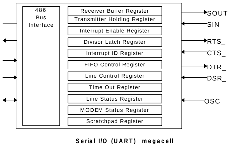
FIGURE 7.6 SERIAL I/O (UART) WITH FIFO
