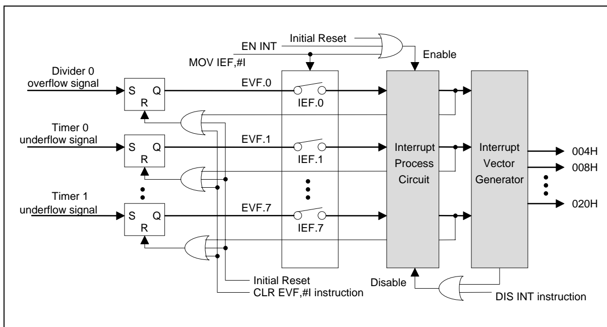
Figure 13. Interrupt event control diagram
