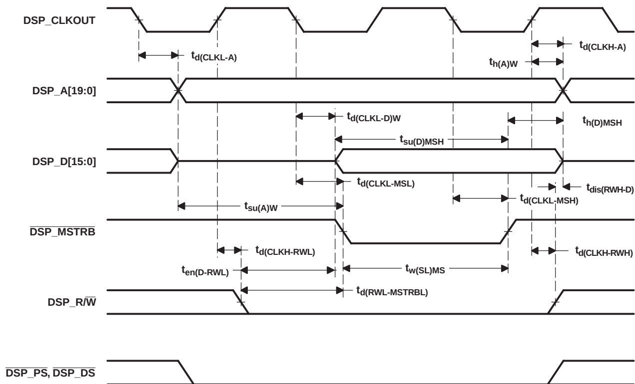
Figure 6–5. Memory Write ( \overline{\text{DSP\_MSTRB}} = 0 )
