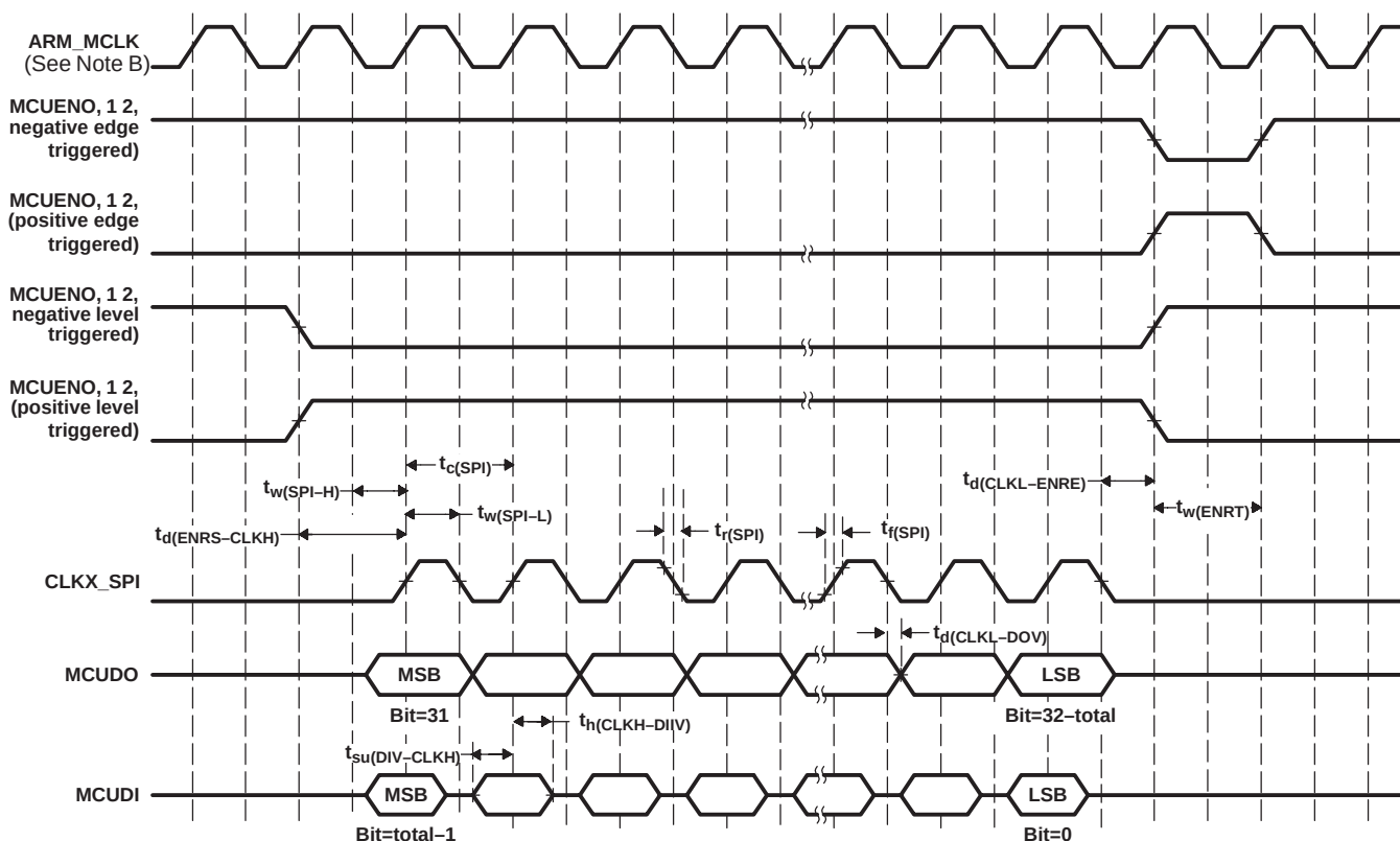
Figure 6–36. SPI Rising Edge Timings
