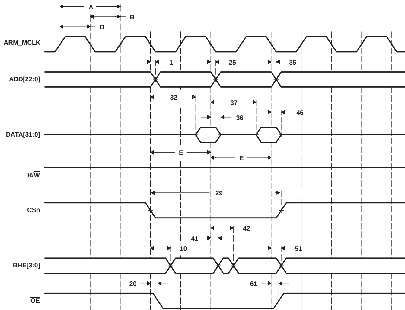
Figure 6–34. ARM SRAM Read Timing
