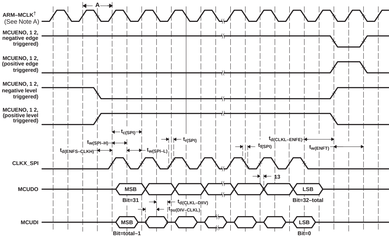
Figure 6–35. SPI Falling Edge Timings
