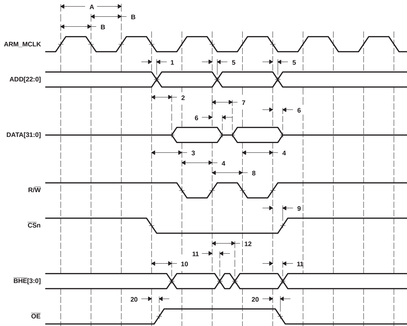
Figure 6–33. ARM SRAM Write Timing
