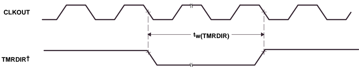
Figure 30. Capture/TMRDIR Timing
