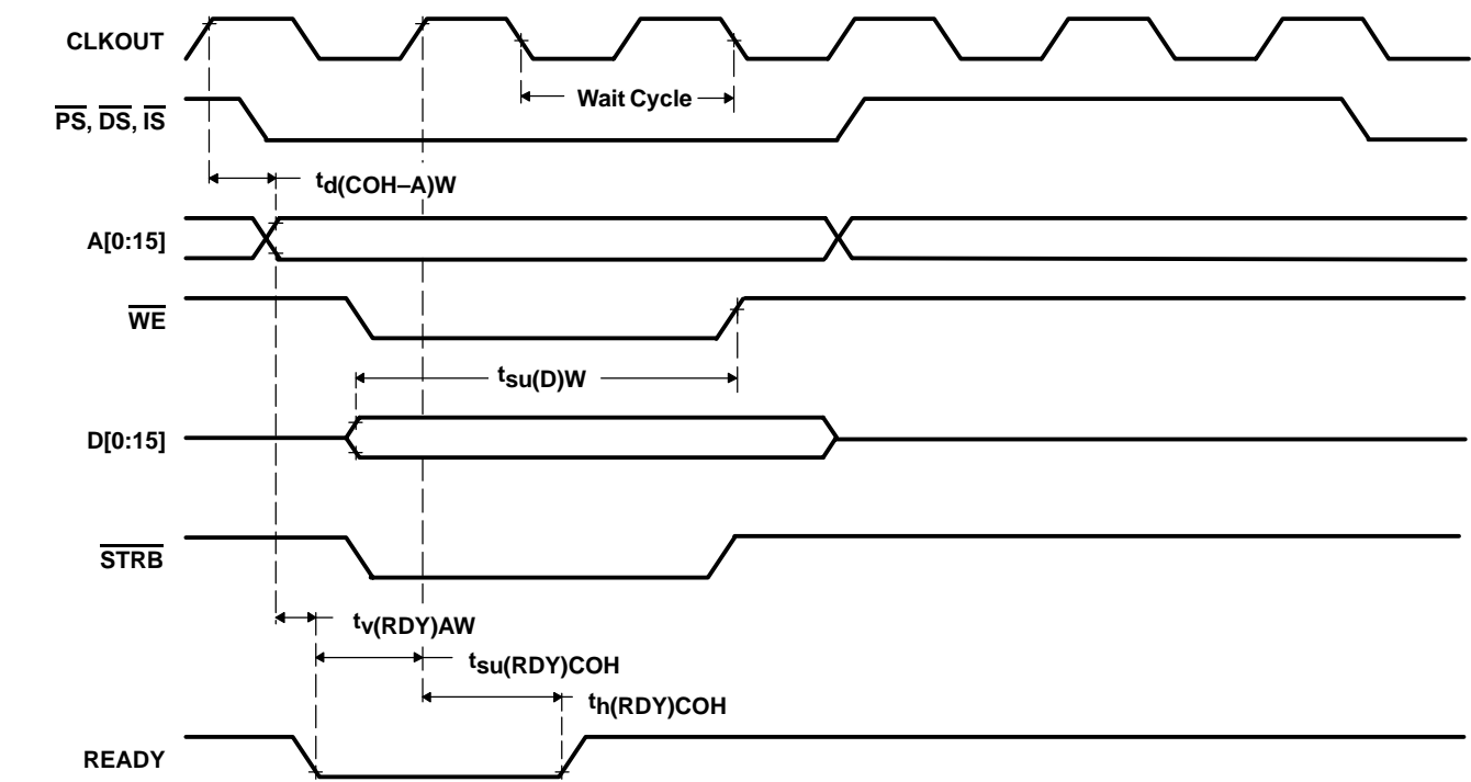
Figure 43. Ready-on-Write Timings
