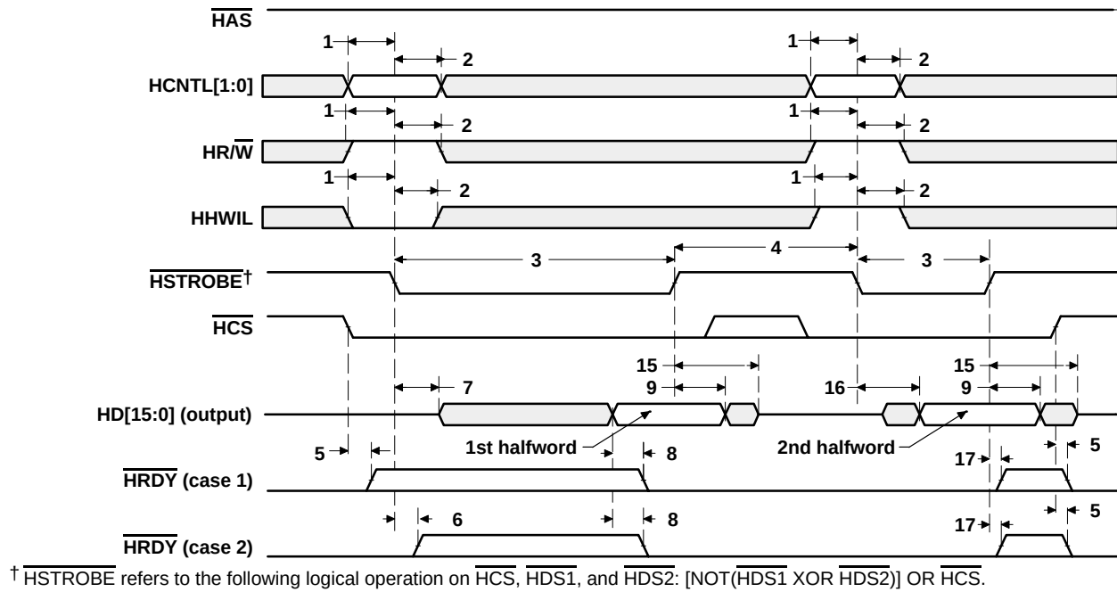
Figure 31. HPI Read Timing ( \overline{HAS} Not Used, Tied High)
