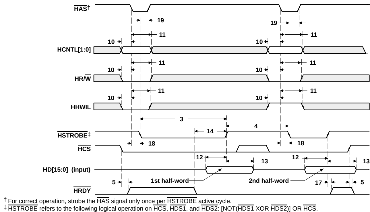
Figure 34. HPI Write Timing ( \overline{HAS} Used)
