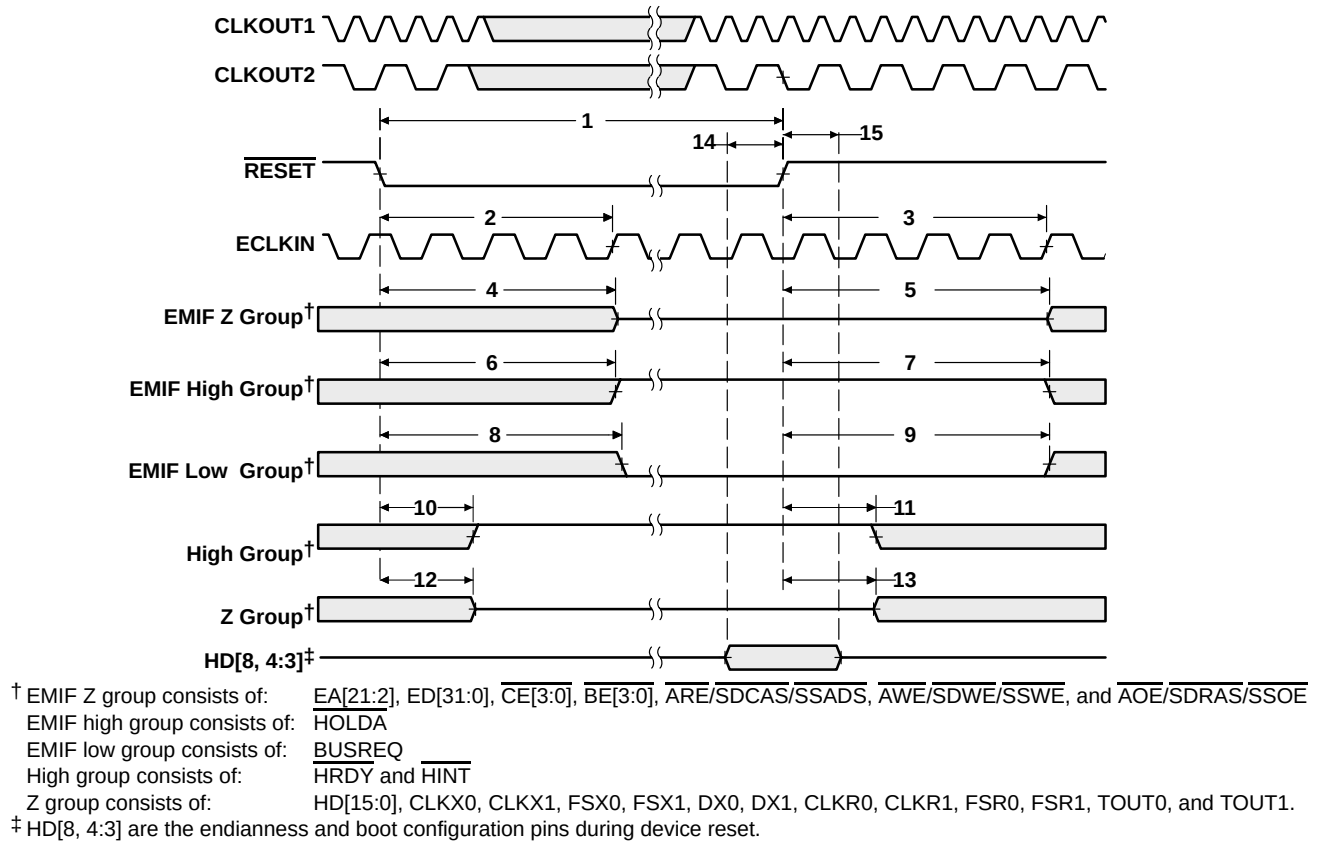
Figure 29. Reset Timing
