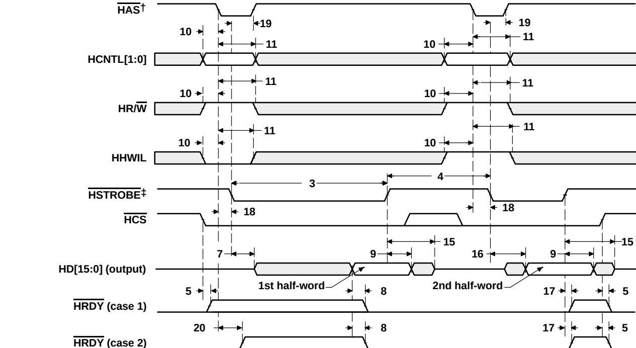
Figure 32. HPI Read Timing ( \overline{HAS} Used)
