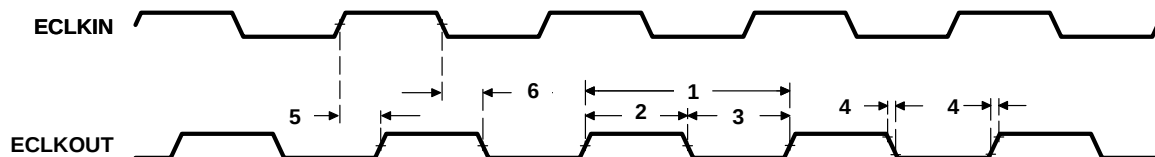
Figure 15. ECLKOUT Timings
