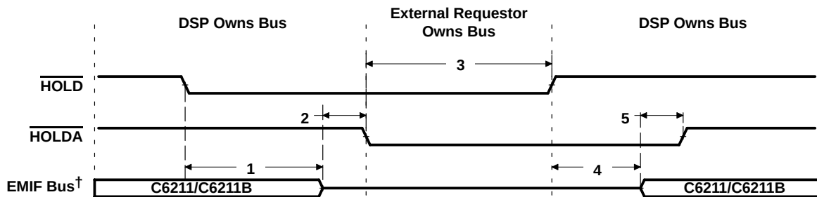
Figure 27. HOLD/HOLDA Timing
