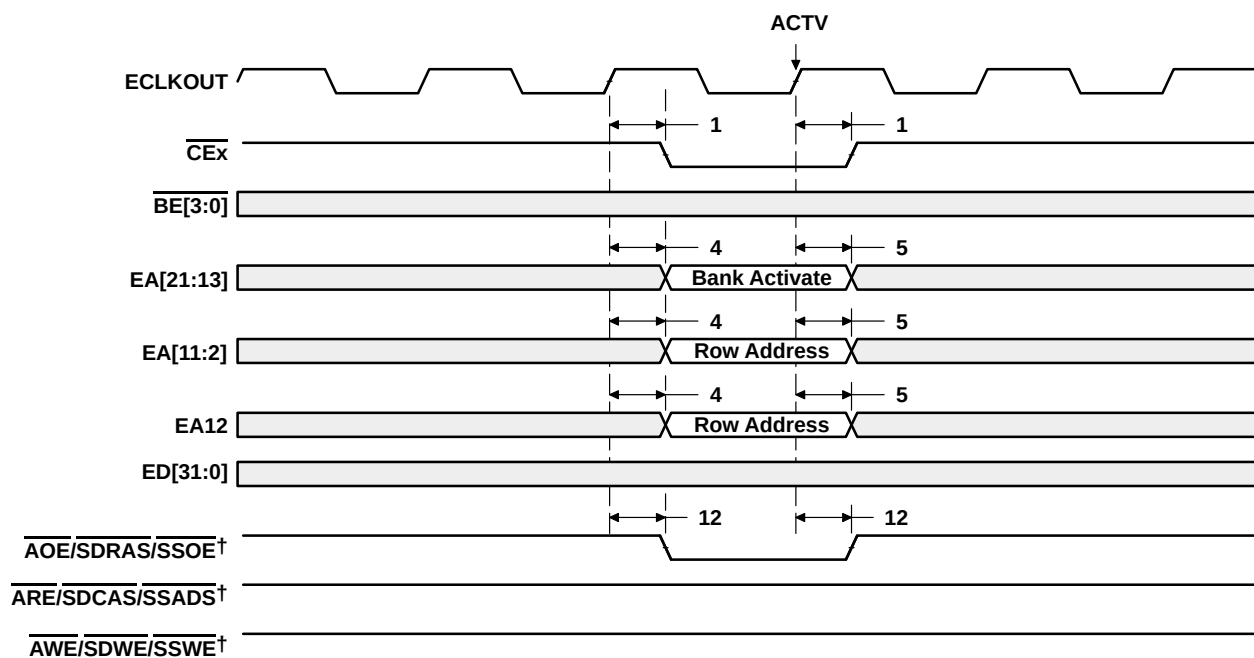
Figure 22. SDRAM ACTV Command
