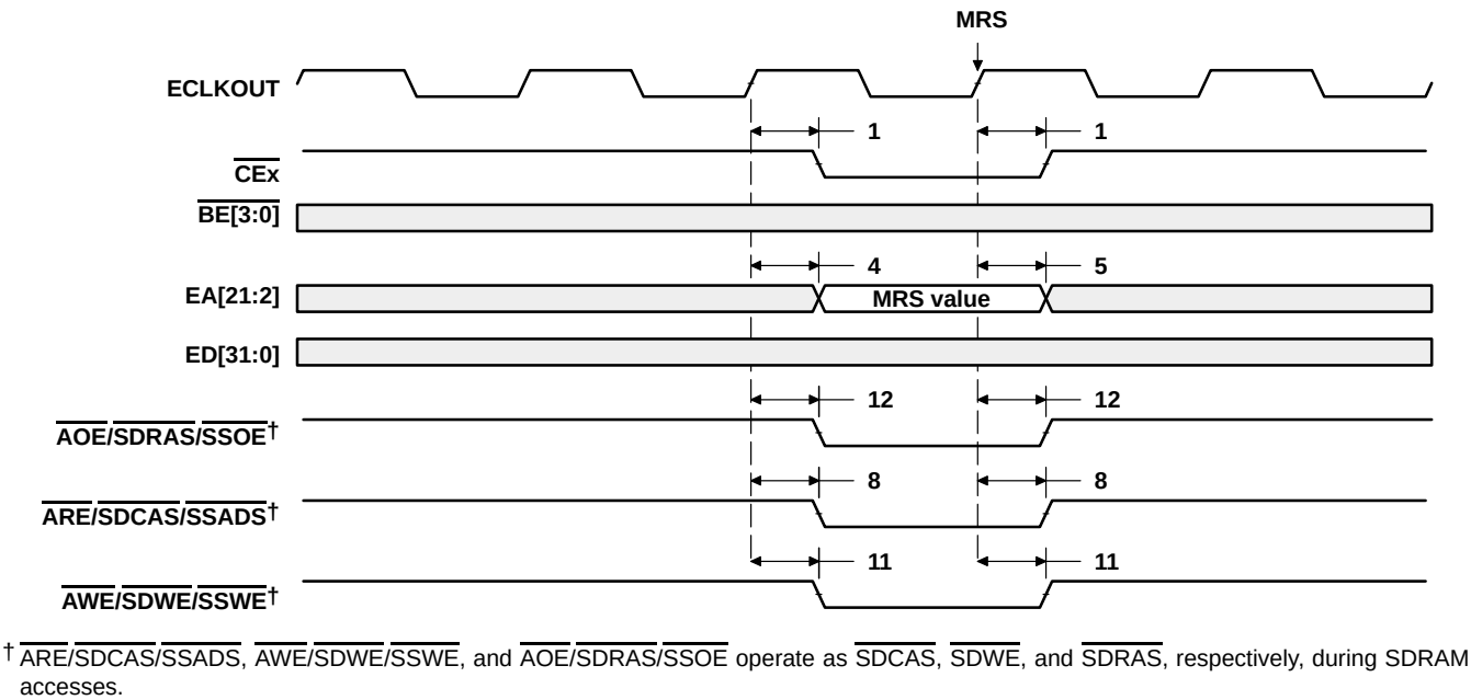
Figure 26. SDRAM MRS Command
