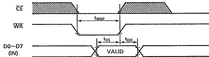
Data Write (1)
