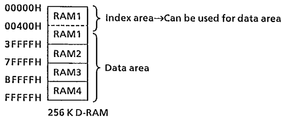
Fig.5.7 Memory map at direct mode
