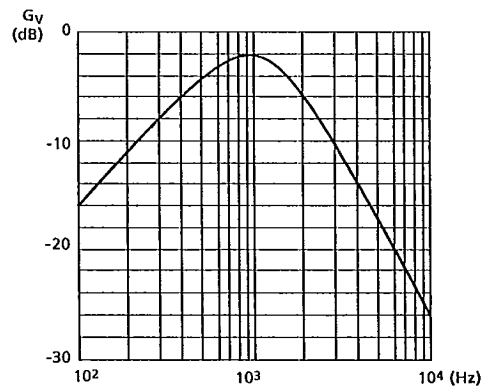
Fig.5.27 Frequency characteristics of band pass filter
