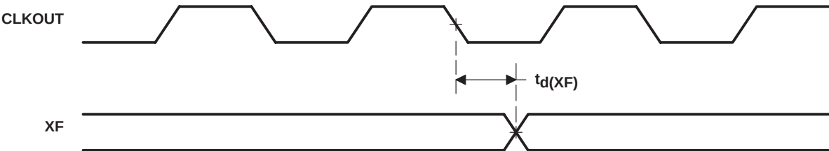
Figure 28. XF Timing
