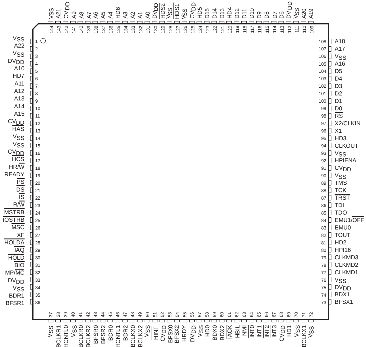
TMS320VC5409 PGE PACKAGE†† (TOP VIEW)
