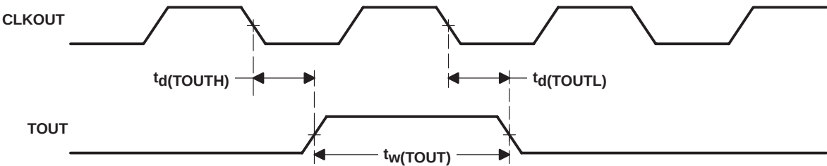
Figure 29. TOUT Timing
