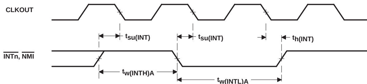
Figure 25. Interrupt Timing
