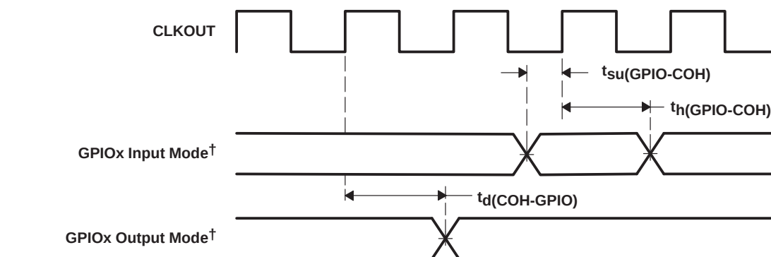
Figure 41. GPIOx † Timings
