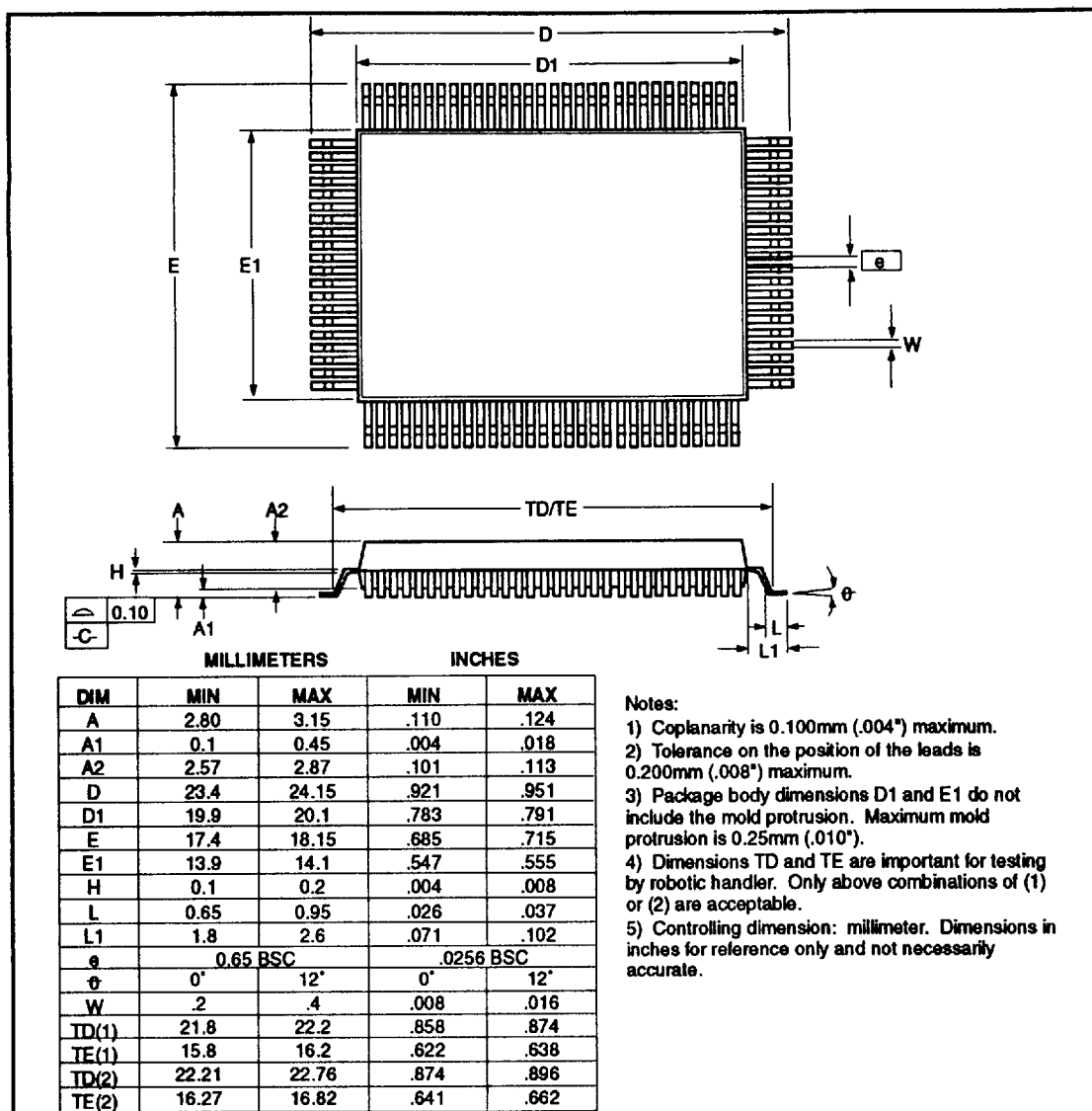
FIGURE 30 - 100 PIN QFP PACKAGE OUTLINES
