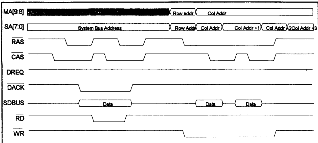
FIGURE 26 - DMA TRANSFER CYCLE TIMING
