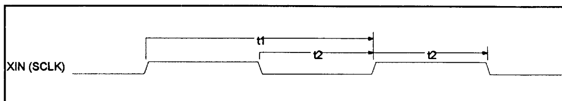
FIGURE 29 - CLOCK TIMING
