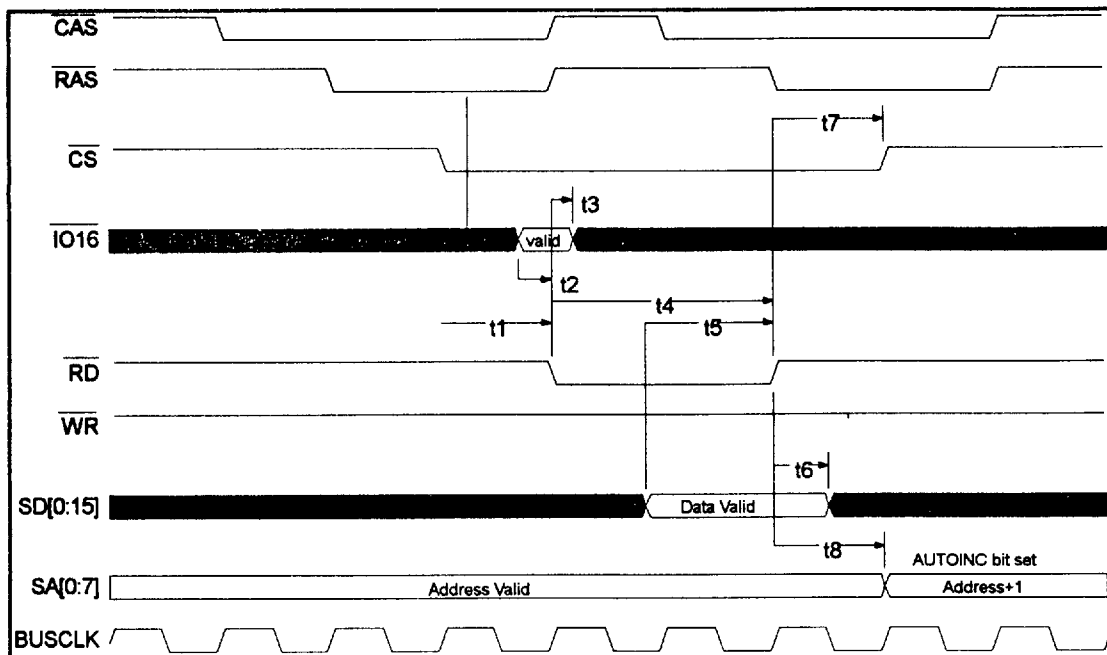
FIGURE 21 - PERIPHERAL BUS READ CYCLE TIMING
