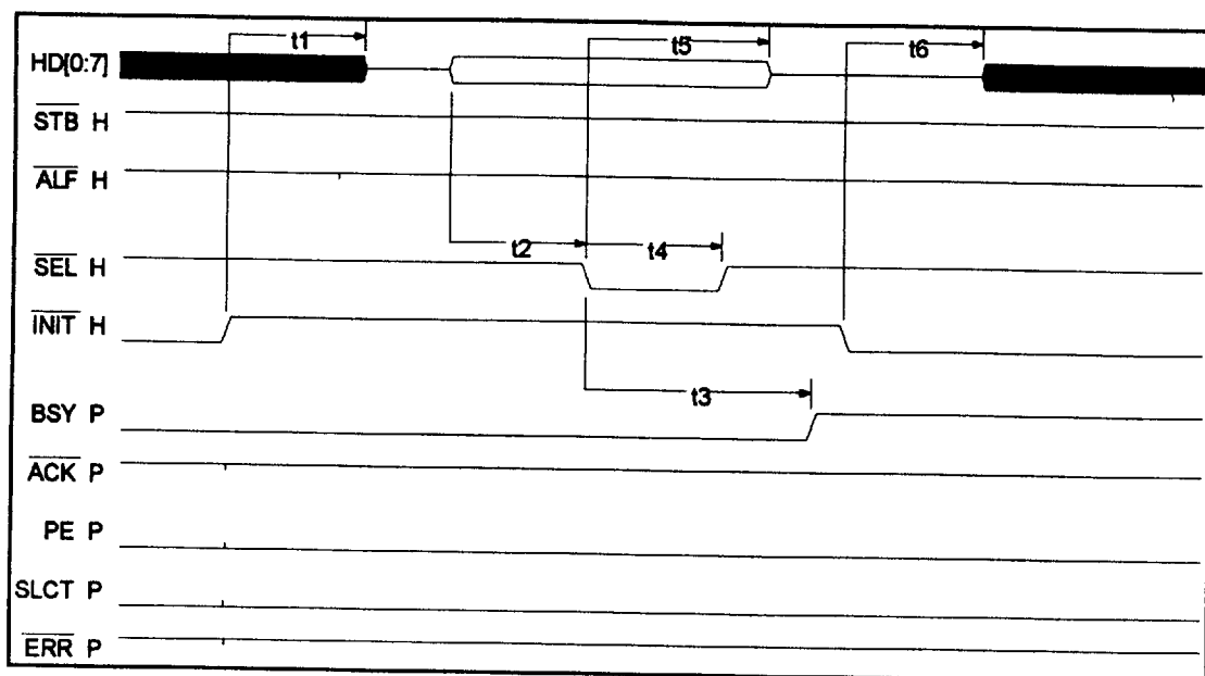
FIGURE 11 - SPP ADDRESS WRITE TIMING (PARALLEL PORT SIGNALS)
