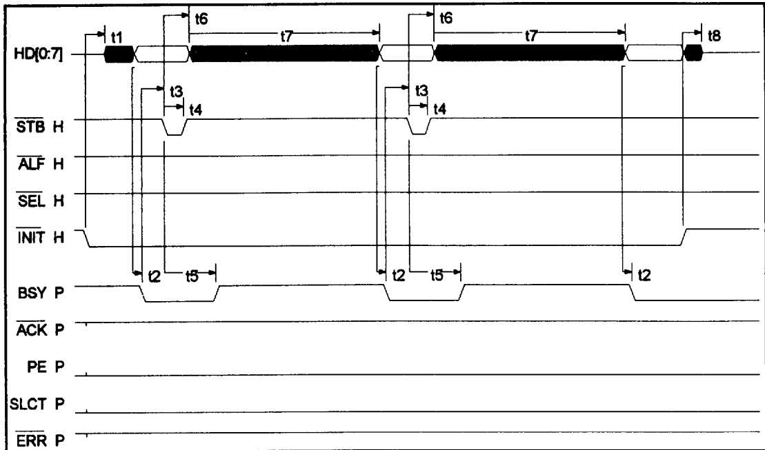
FIGURE 13 - SPP DATA READ TIMING (PARALLEL PORT SIGNALS)
