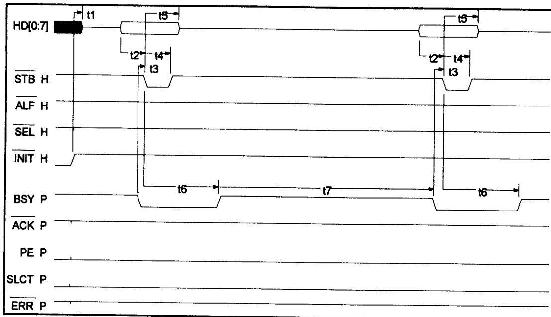
FIGURE 12 - SPP DATA WRITE TIMING (PARALLEL PORT SIGNALS)
