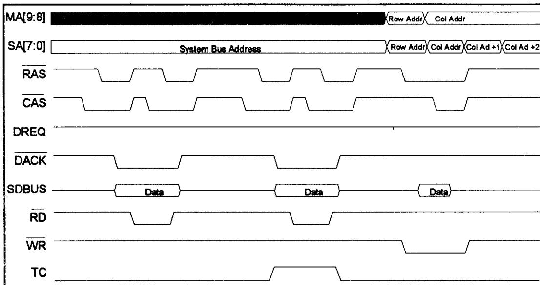
FIGURE 27 - DMA TRANSFER CYCLE TIMING
