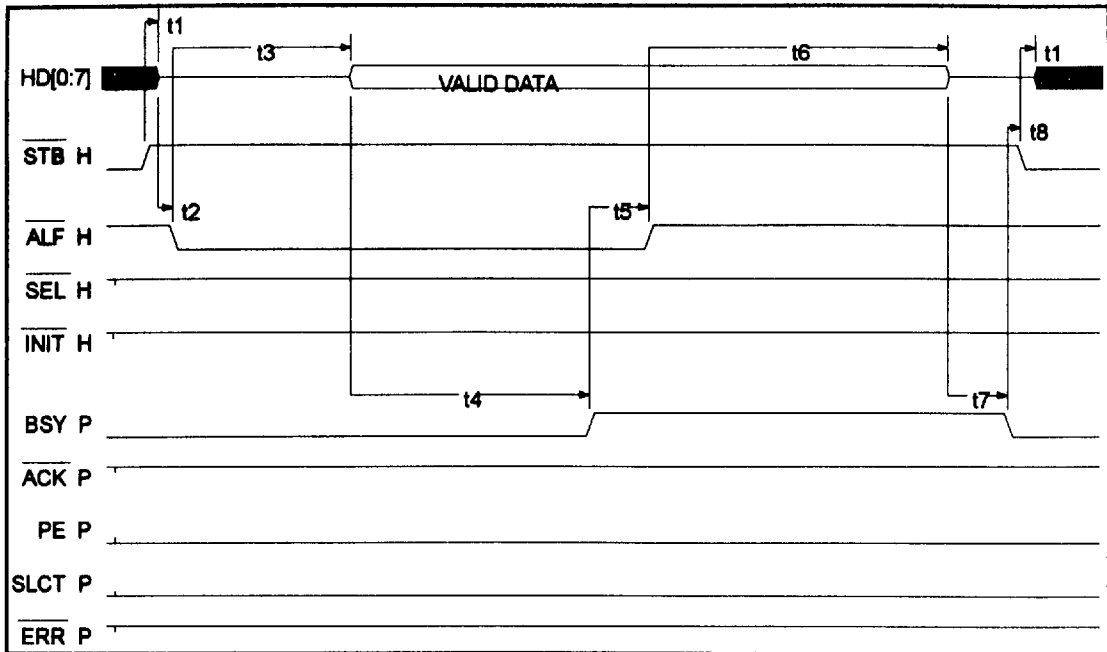
FIGURE 17 - EPP DATA READ TIMING (PARALLEL PORT SIGNALS)
