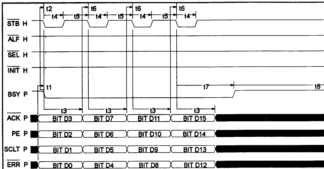
FIGURE 14 - SPP NIBBLE READ (PARALLEL PORT SIGNALS)
