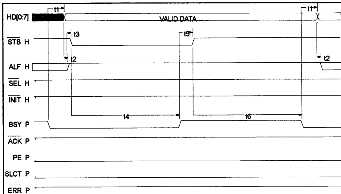
FIGURE 19 - ECP FORWARD DATA TRANSFER TIMING (ECP DATA WRITE, PARALLEL PORT SIGNALS)
