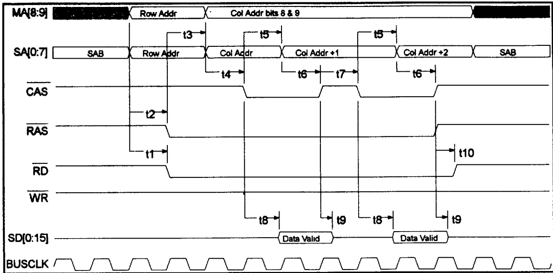
FIGURE 23 - DRAM READ CYCLE TIMING
