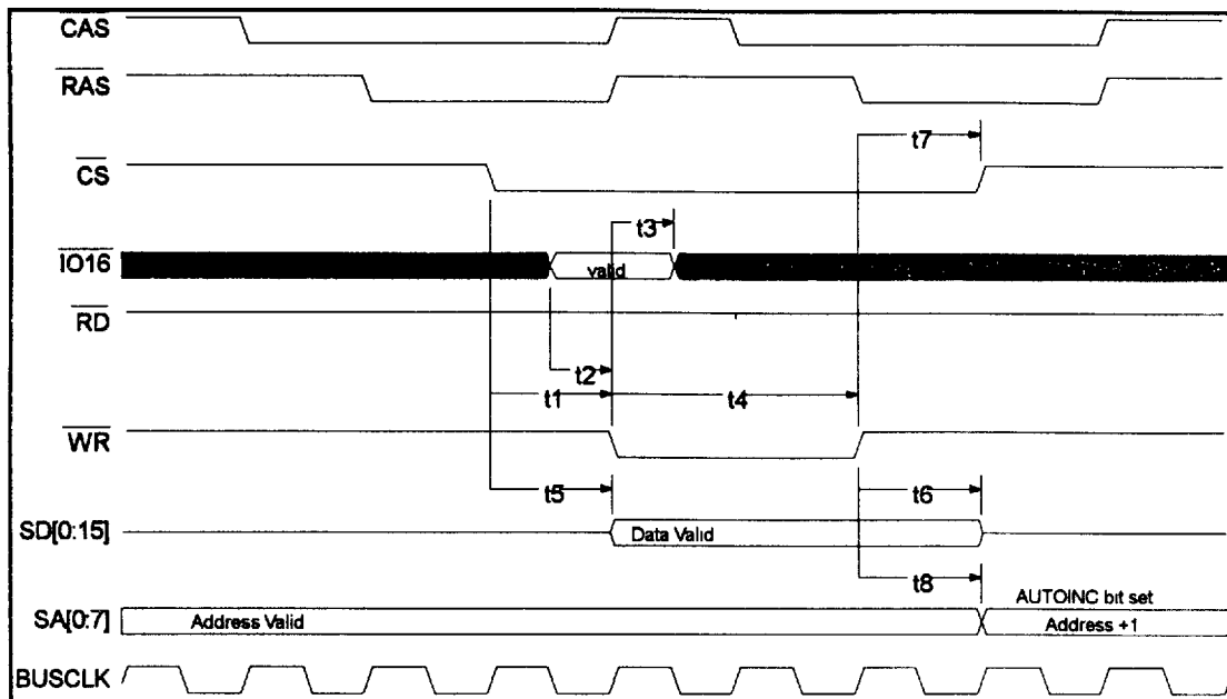
FIGURE 22 - PERIPHERAL BUS WRITE CYCLE TIMING
