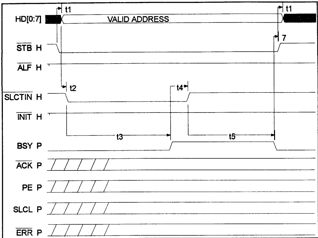
FIGURE 15 - EPP ADDRESS WRITE (PARALLEL PORT SIGNALS)
