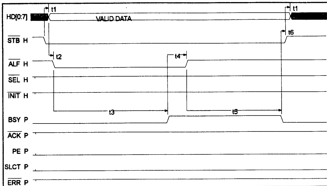
FIGURE 16 - EPP DATA WRITE TIMING (PARALLEL PORT SIGNALS)
