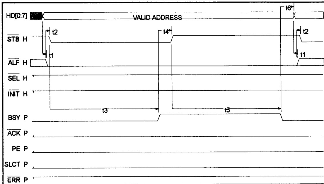
FIGURE 18 - ECP FORWARD COMMAND TRANSFER TIMING (ECP ADDRESS WRITE, PARALLEL PORT SIGNALS)
