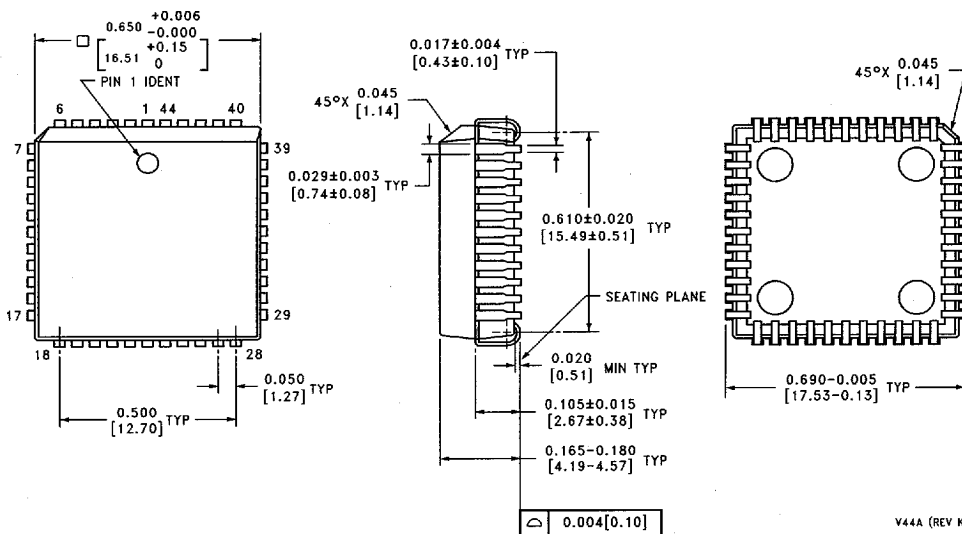
44-Lead Plastic Chip Carrier (V) Order Number PC16552DV NS Package Number V44A
