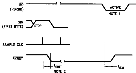
Receiver Ready FCR0 = 0 or FCR0 = 1 and FCR3 = 0 (Mode 0)
