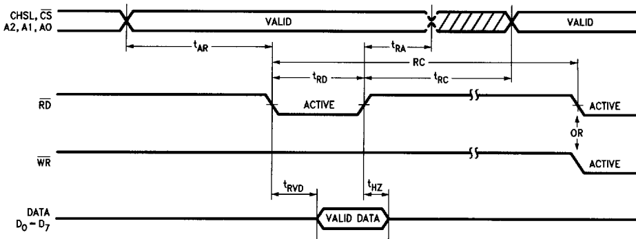
Read Cycle
