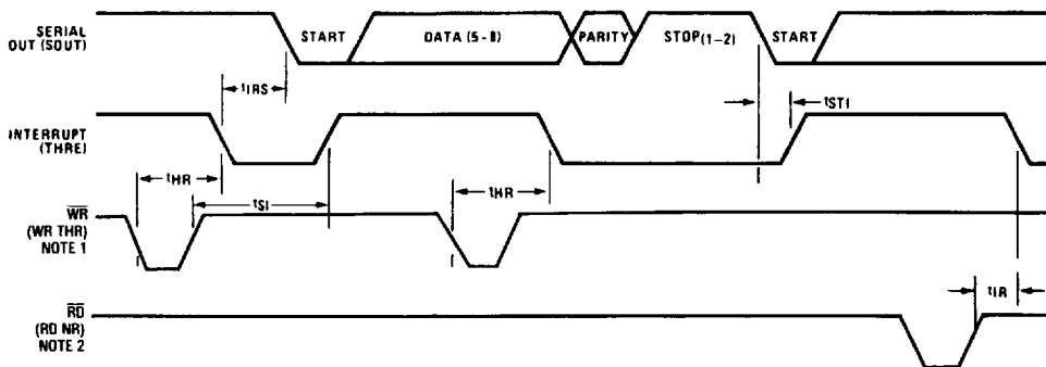
Transmitter Timing
