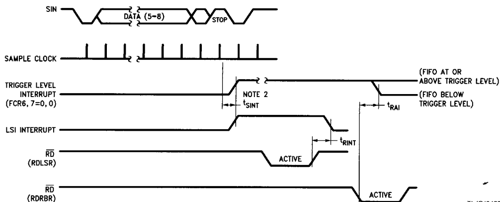
RCVR FIFO First Byte (This Sets RDR)
