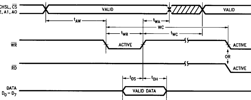
Write Cycle
