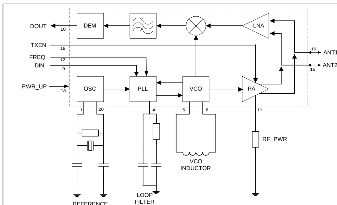
Figure 1. nRF403 block diagram with external components.
