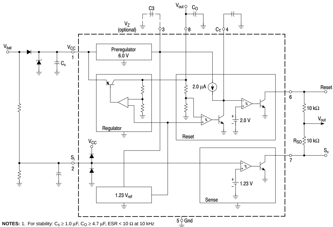
Figure 11. Application Schematic
