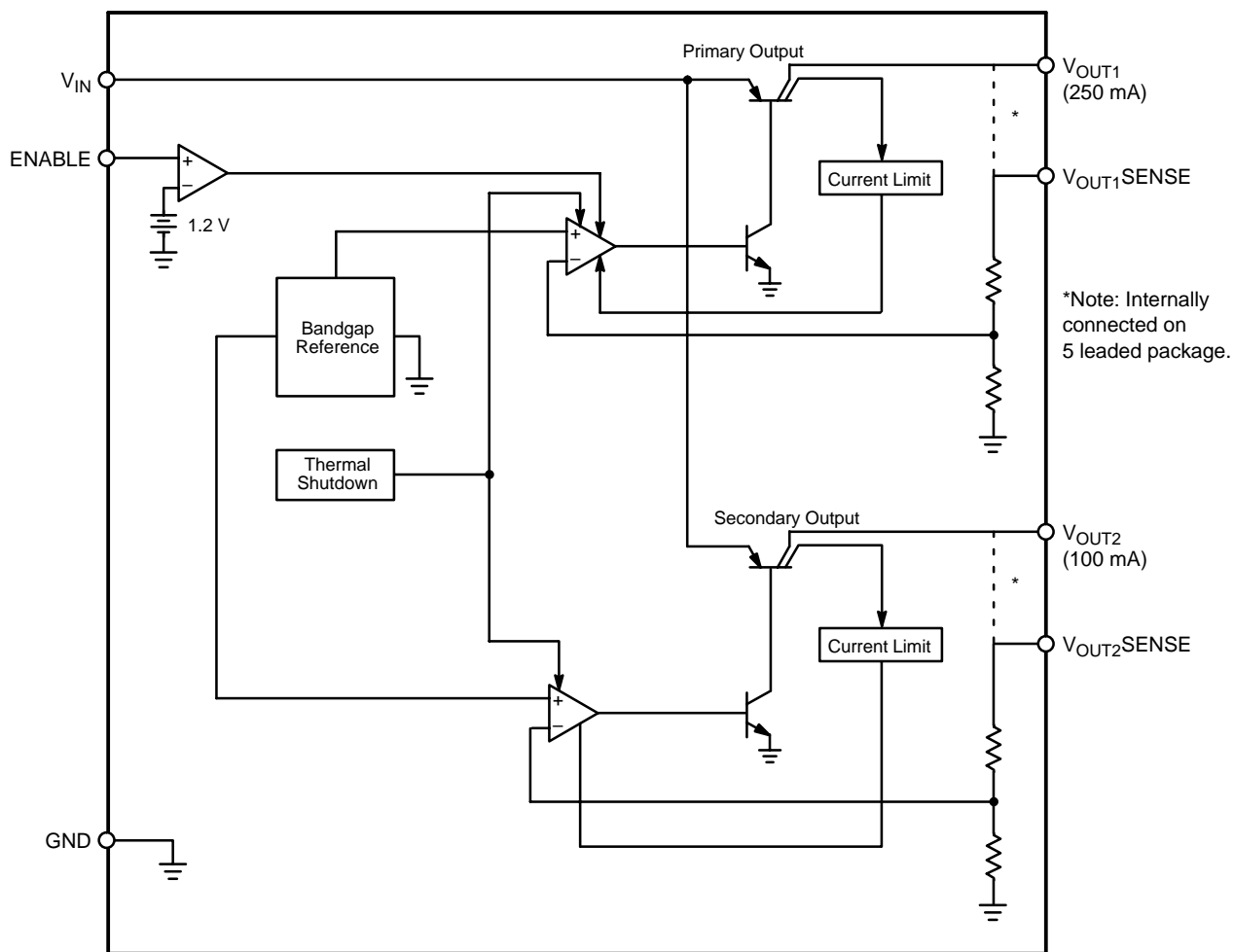
Figure 1. Block Diagram
