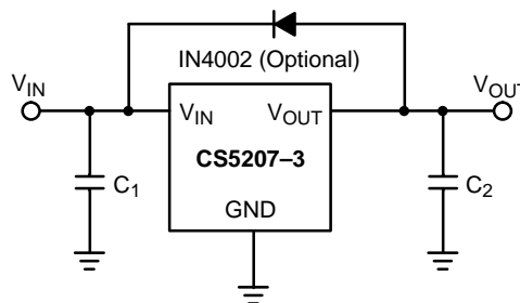
Figure 6. Protection Diode Scheme for Fixed Output Regulator
