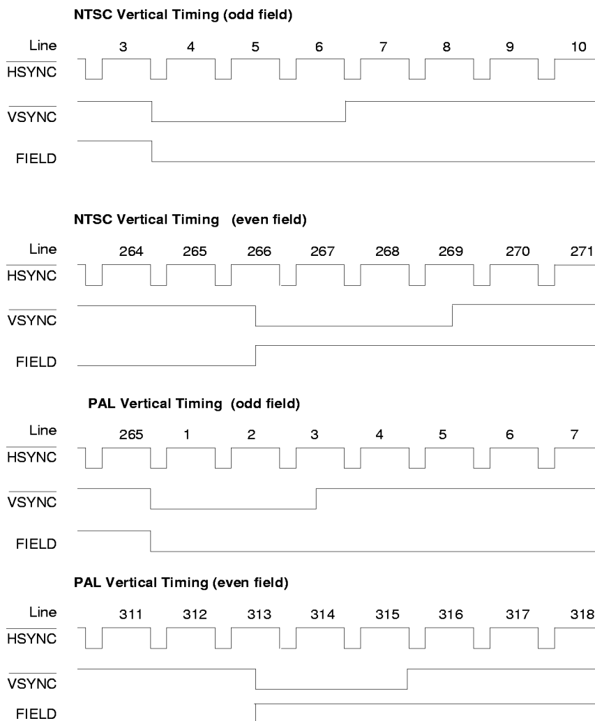
Figure 6. Vertical Timing
