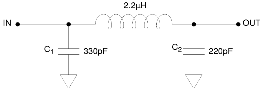
Figure 30. External Low Pass Filter C_2 should be chosen so that C_1 = C_2 + C_{\text{cable}}
