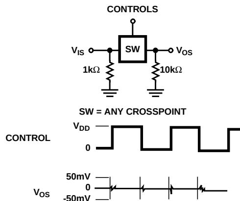
FIGURE 6. TEST CIRCUIT AND WAVEFORMS FOR CROSSTALK (CONTROL INPUT TO SIGNAL OUTPUT)
