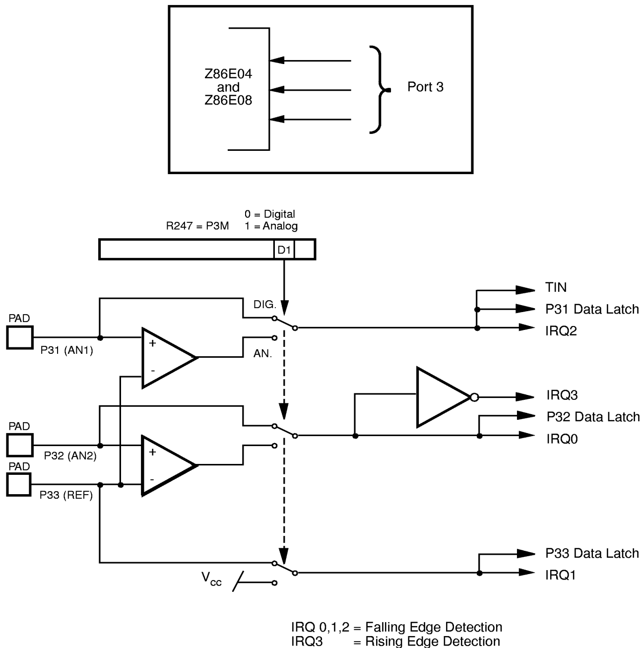
Figure 9. Port 3 Configuration
