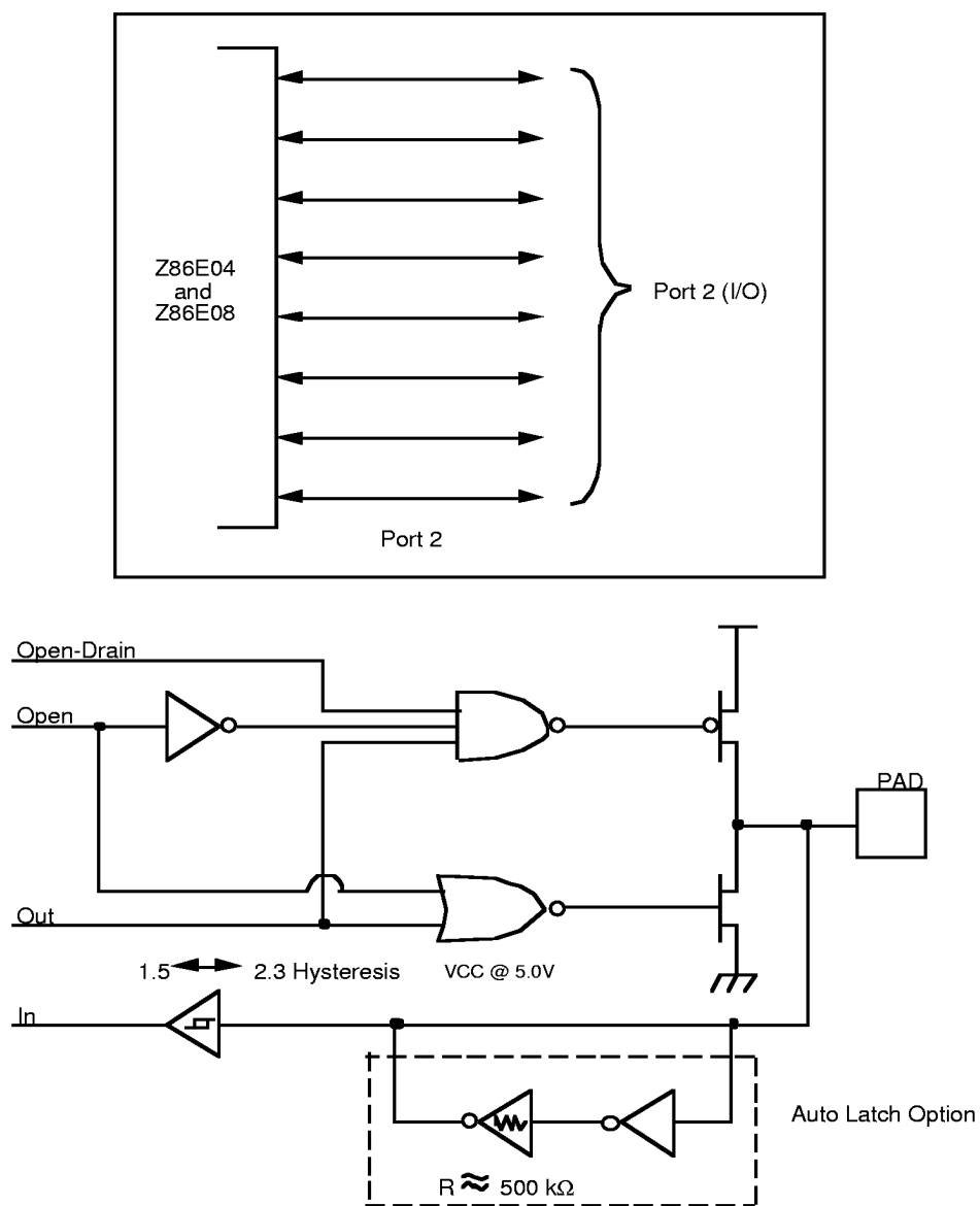
Figure 8. Port 2 Configuration
