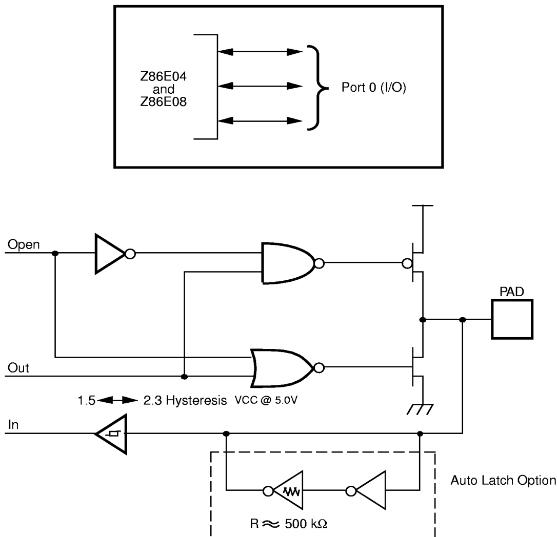
Figure 7. Port 0 Configuration
