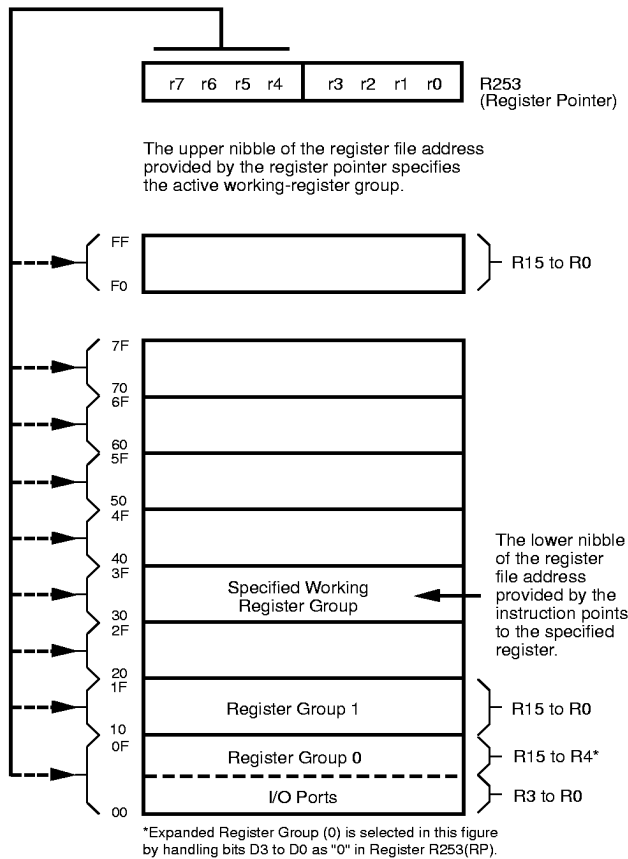
Figure 13. Register Pointer
