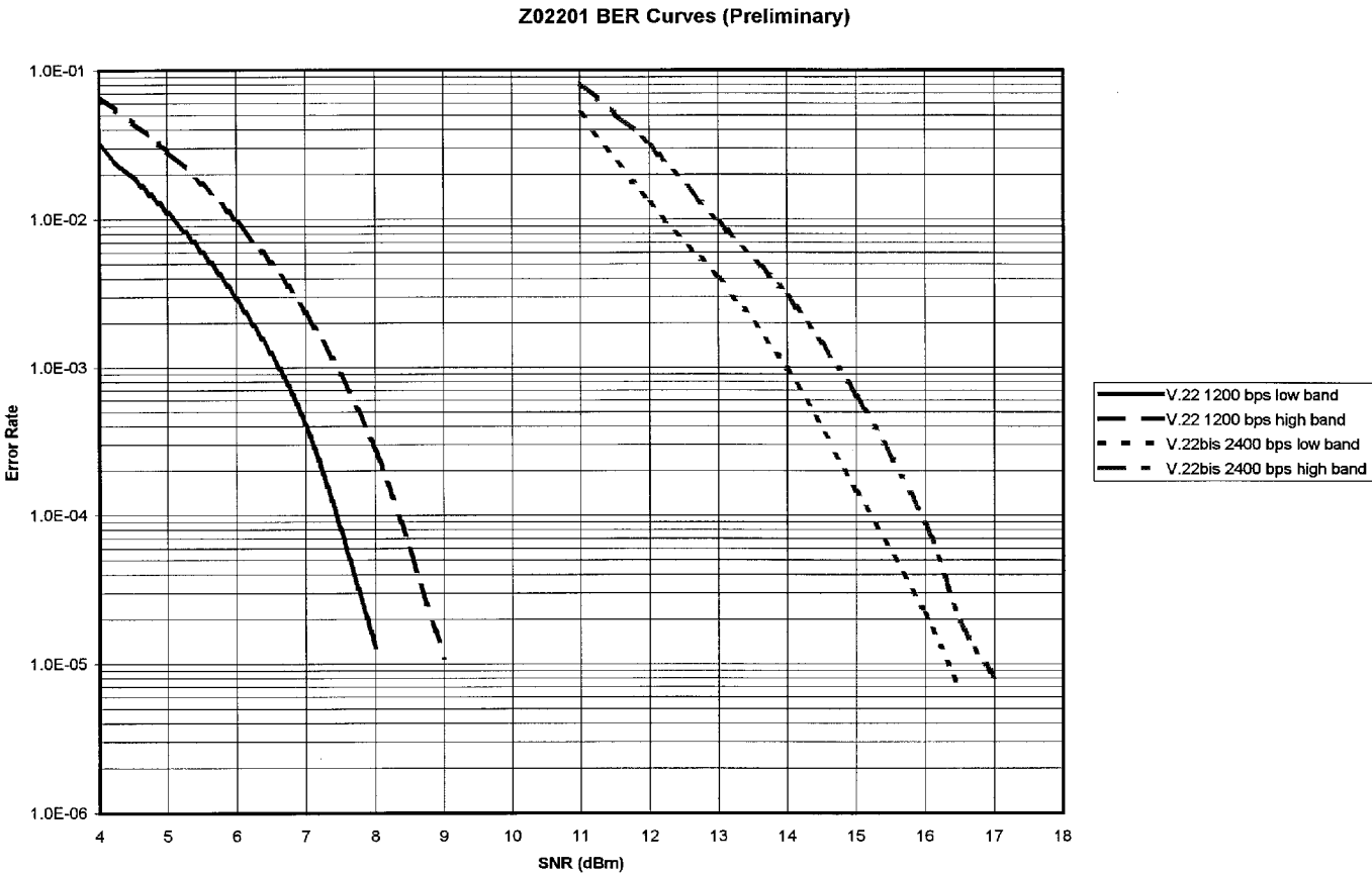
Figure 9. Typical Performance Data
