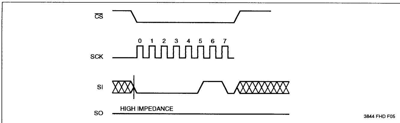
Figure 2. Write Enable Latch
