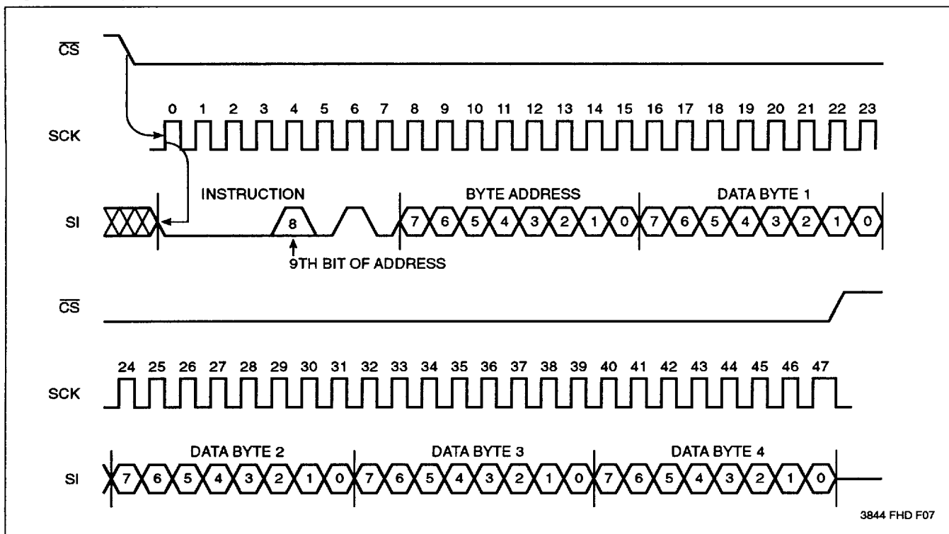
Figure 4. Page Write Operation Sequence
