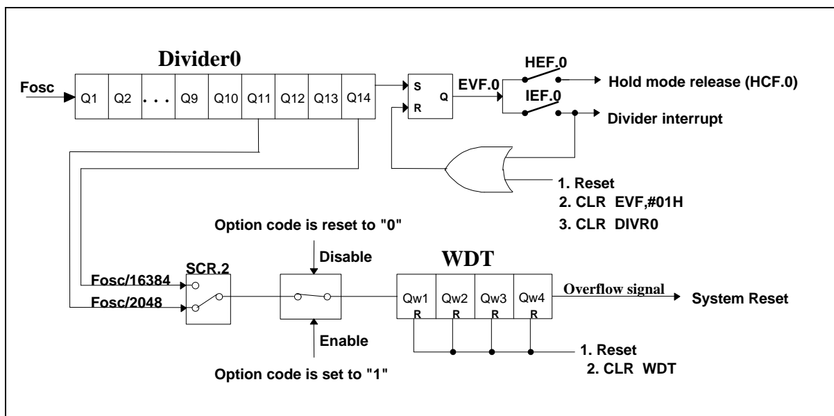
Figure 5-5 Organization of Divider0 and watchdog timer
