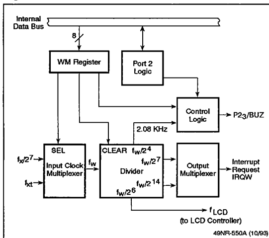
Figure 10. Watch Timer
