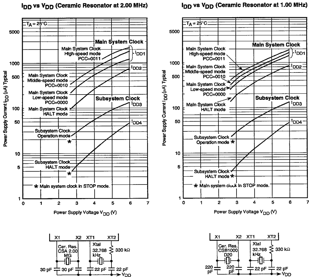
Figure 19. DC Characteristics, I_{DD} vs V_{DD} ( \mu PD7530x/31x, Standard Grade) (Sheet 2 of 2)
