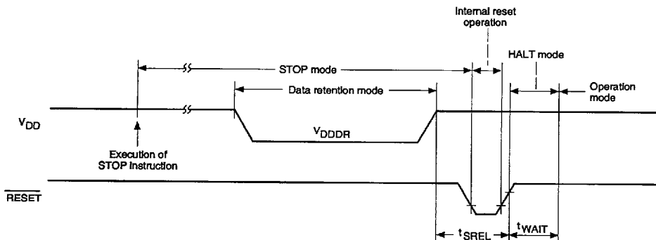
Figure 29. Low-Voltage Data Retention Timing
