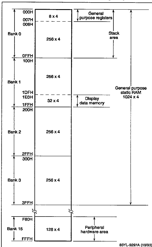
Figure 3. μPD75P316A Data Memory Map
