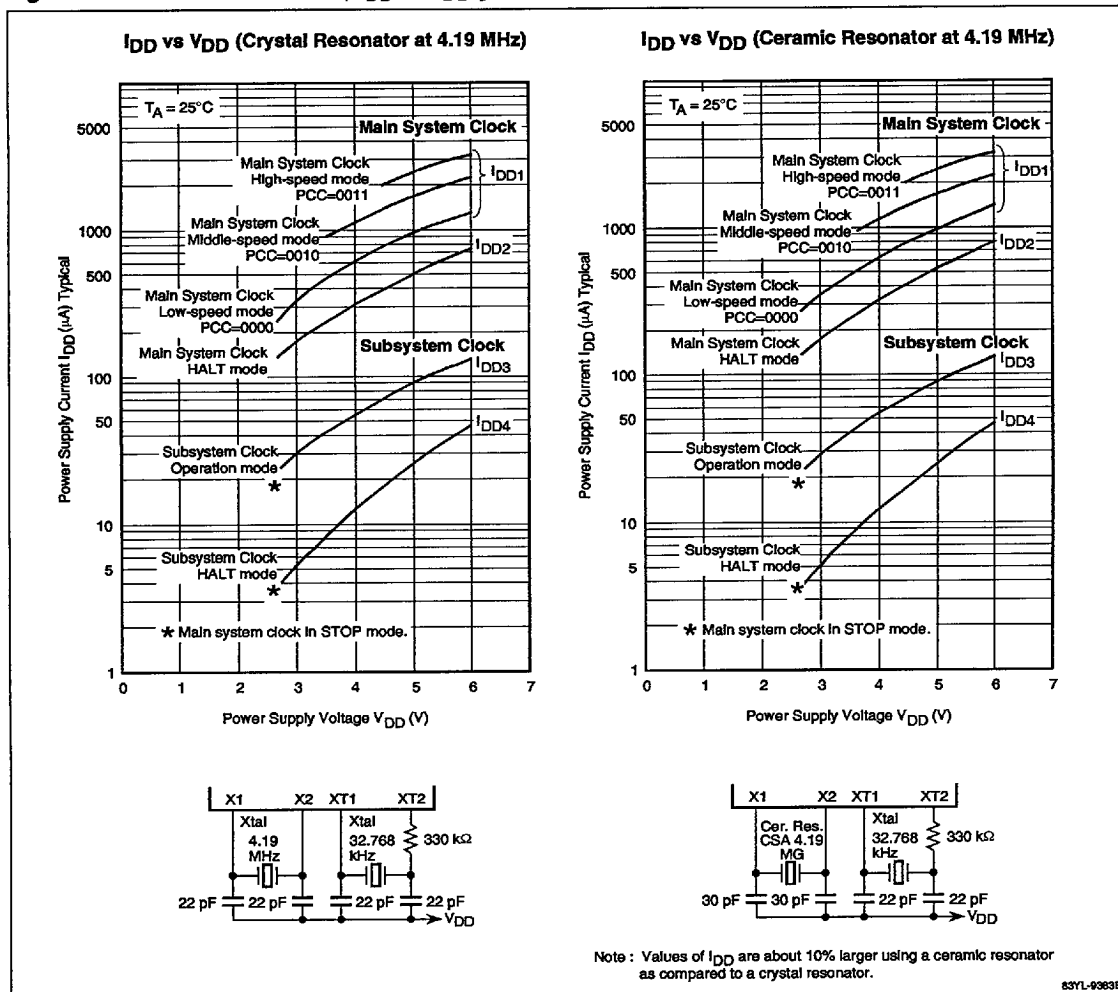
Figure 19. DC Characteristics, I_{DD} vs V_{DD} (μPD7530x/31x, Standard Grade) (Sheet 1 of 2)
