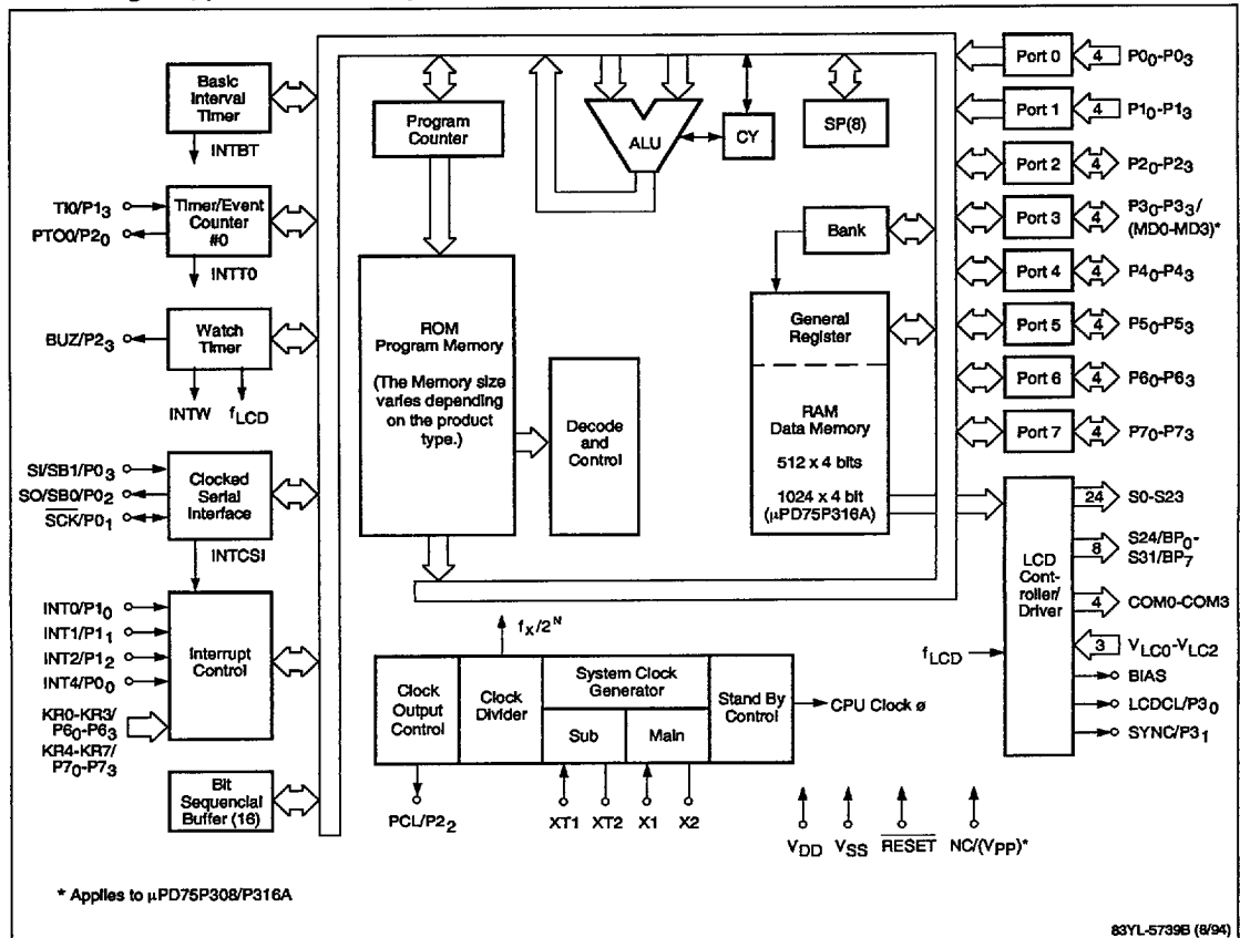
Block Diagram; μPD75316 Family
