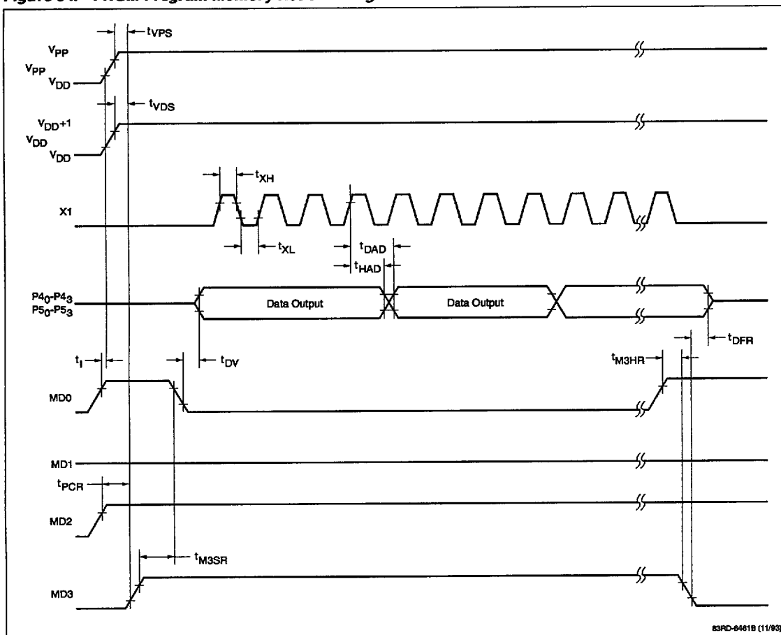
Figure 34. PROM Program Memory Read Timing
