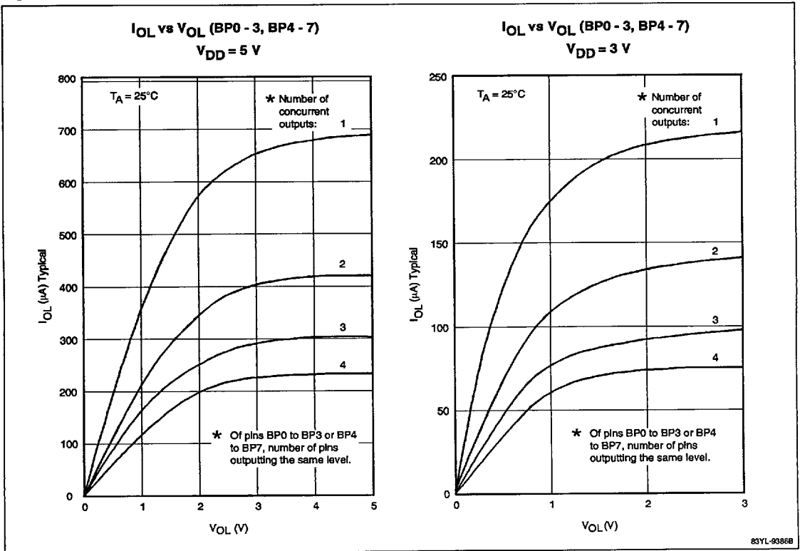
Figure 20. DC Characteristics, I_{OL} vs V_{OL} ( \mu PD7530x/31x, Standard Grade) (Sheet 2 of 2)
