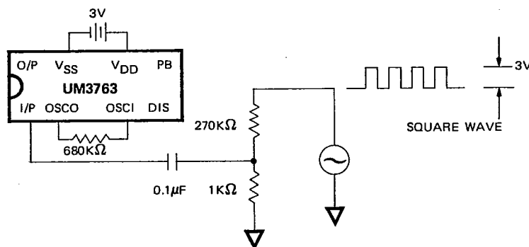
Figure 2. Circuit
