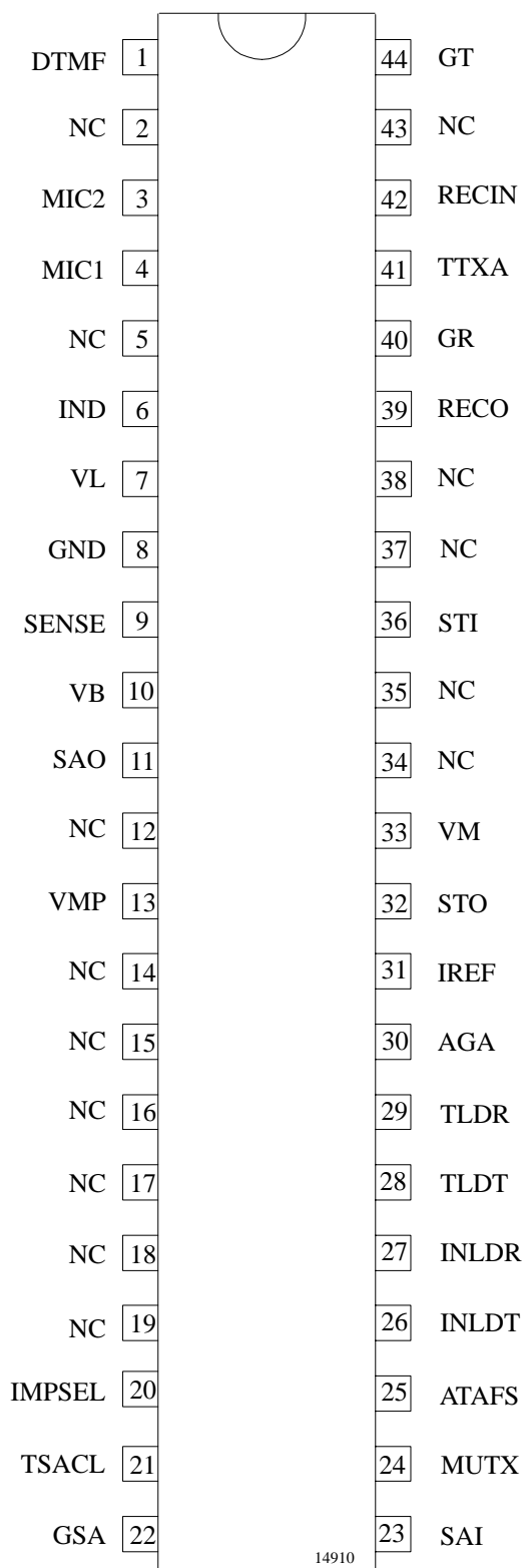
Figure 4. Pinning SSO44
