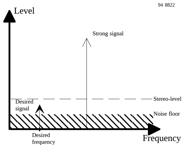
Figure 3 A low AGC threshold causes the blocking signal to suppress the desired signal
