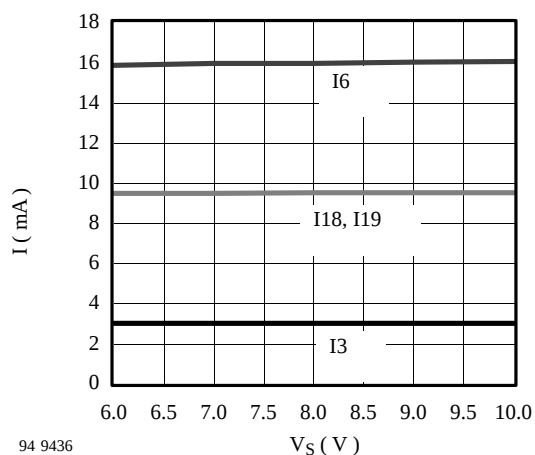
Supply currents versus supply voltage
