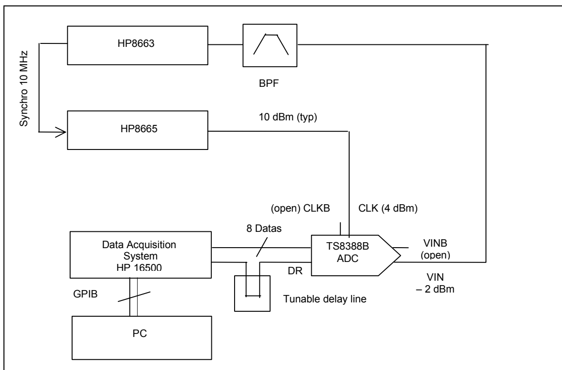
Figure 15 : SINGLE-ENDED ANALOG AND CLOCK INPUT CONFIGURATION
