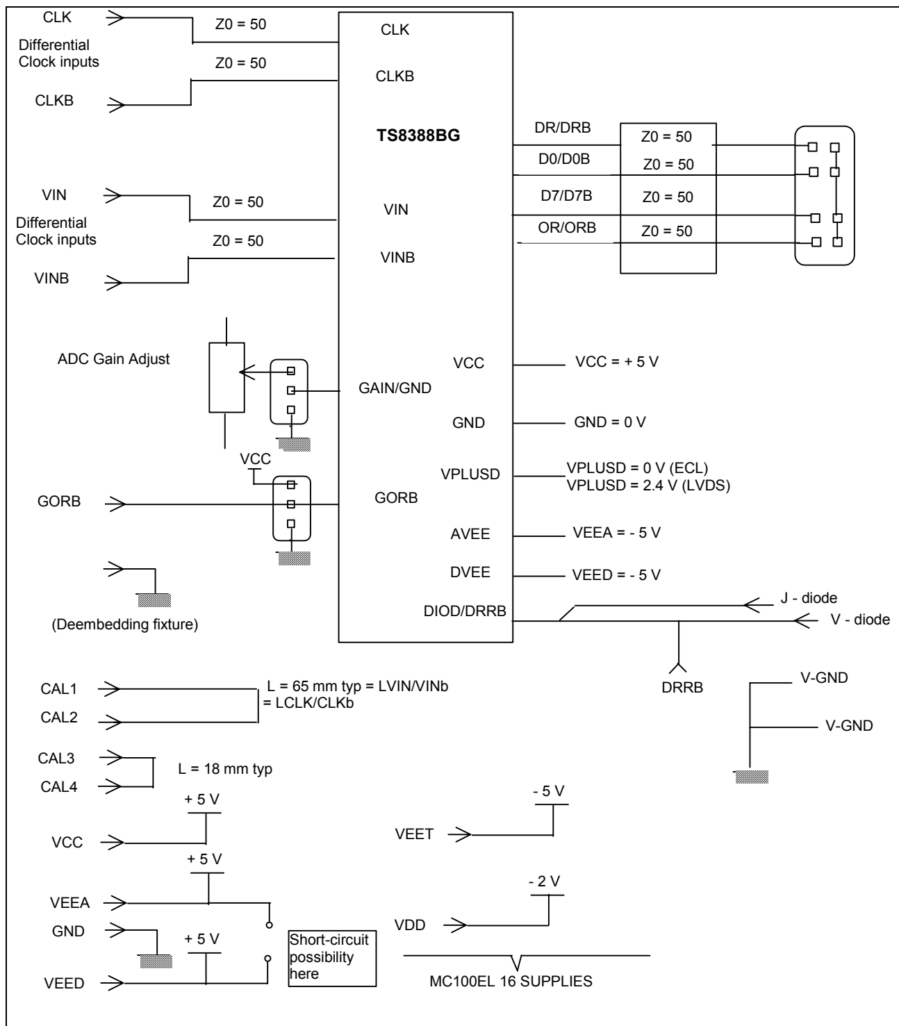
Figure 1 : TSEV8388BG BLOCK DIAGRAM
