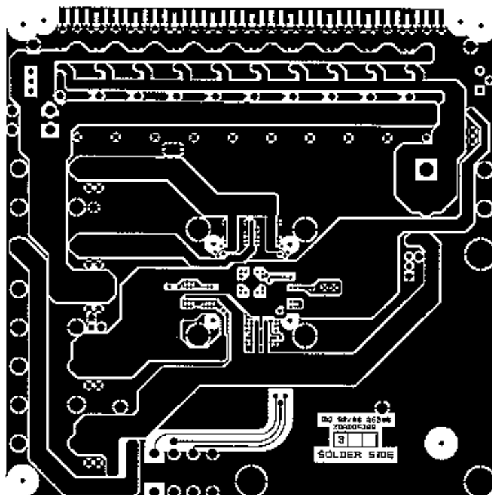
Figure 10 : POWER SUPPLIES PLANES
