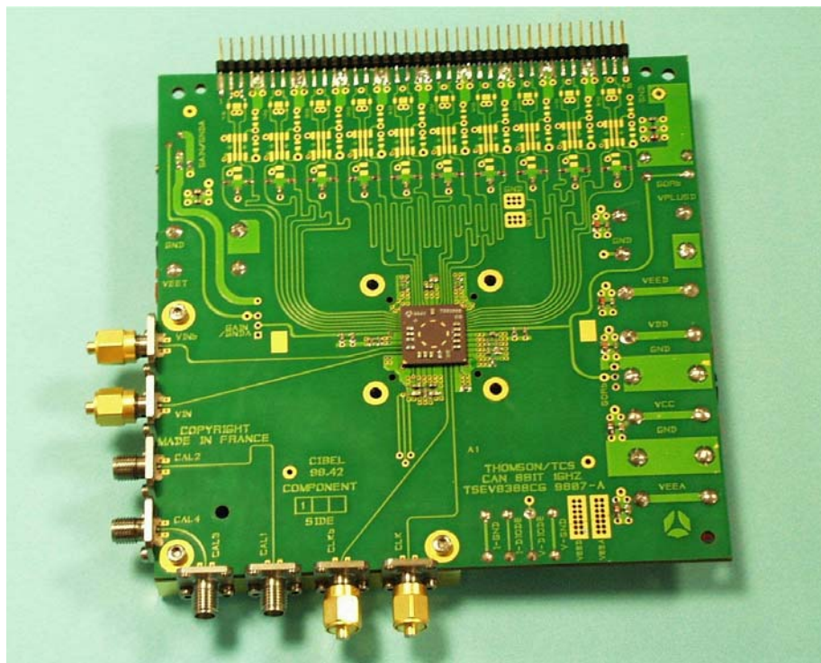
Figure 12 : TSEV8388BG EVALUATION BOARD : TOP VIEW (SIGNAL SIDE)
