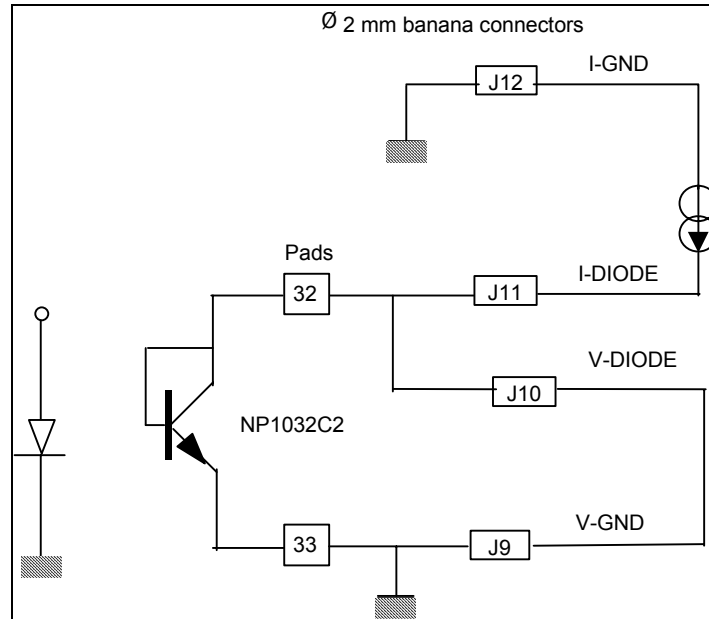
Figure 2 : TS8388BG DIE JUNCTION TEMPERATURE MEASUREMENT SETUP
