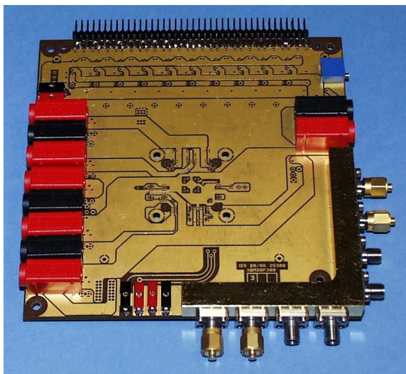
Figure 13 : TSEV8388BG EVALUATION BOARD : BOTTOM VIEW
