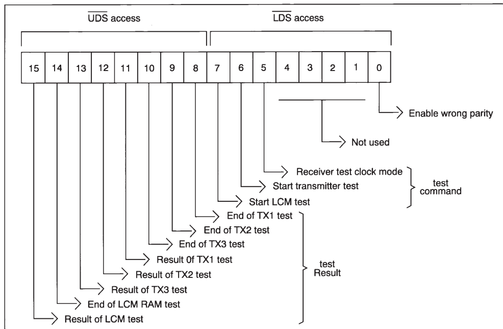
Figure 26 : Self-test register.
