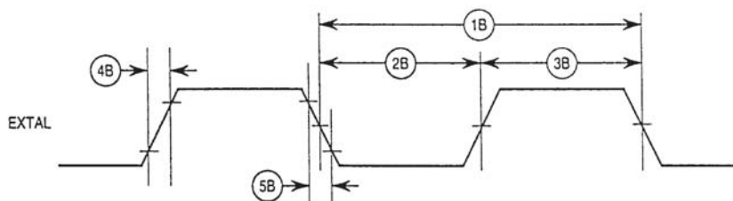
Figure 5. External Input Timing Diagram
