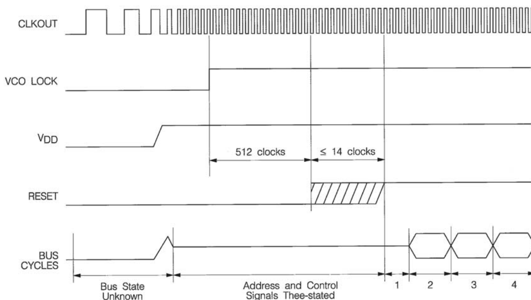
Figure 20. Initial Reset Operation Timing
