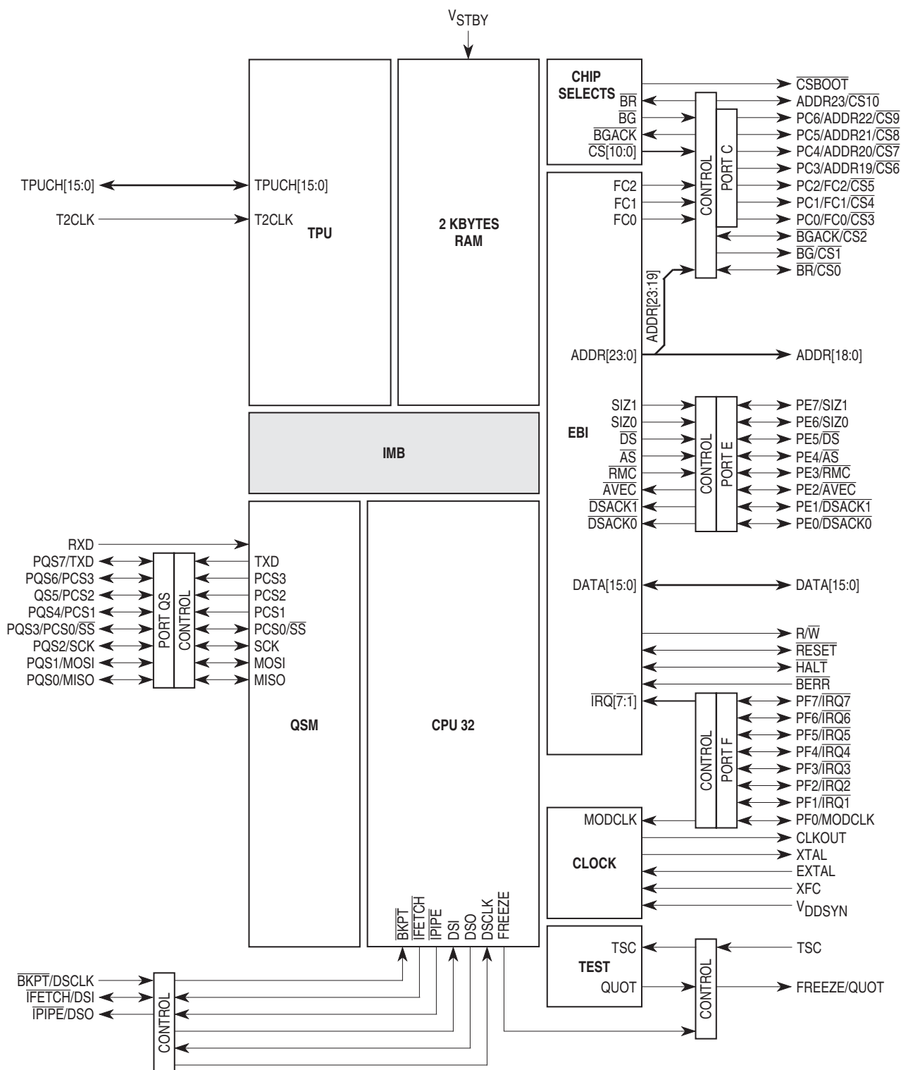
Figure 1. Block Diagram of TS68332
