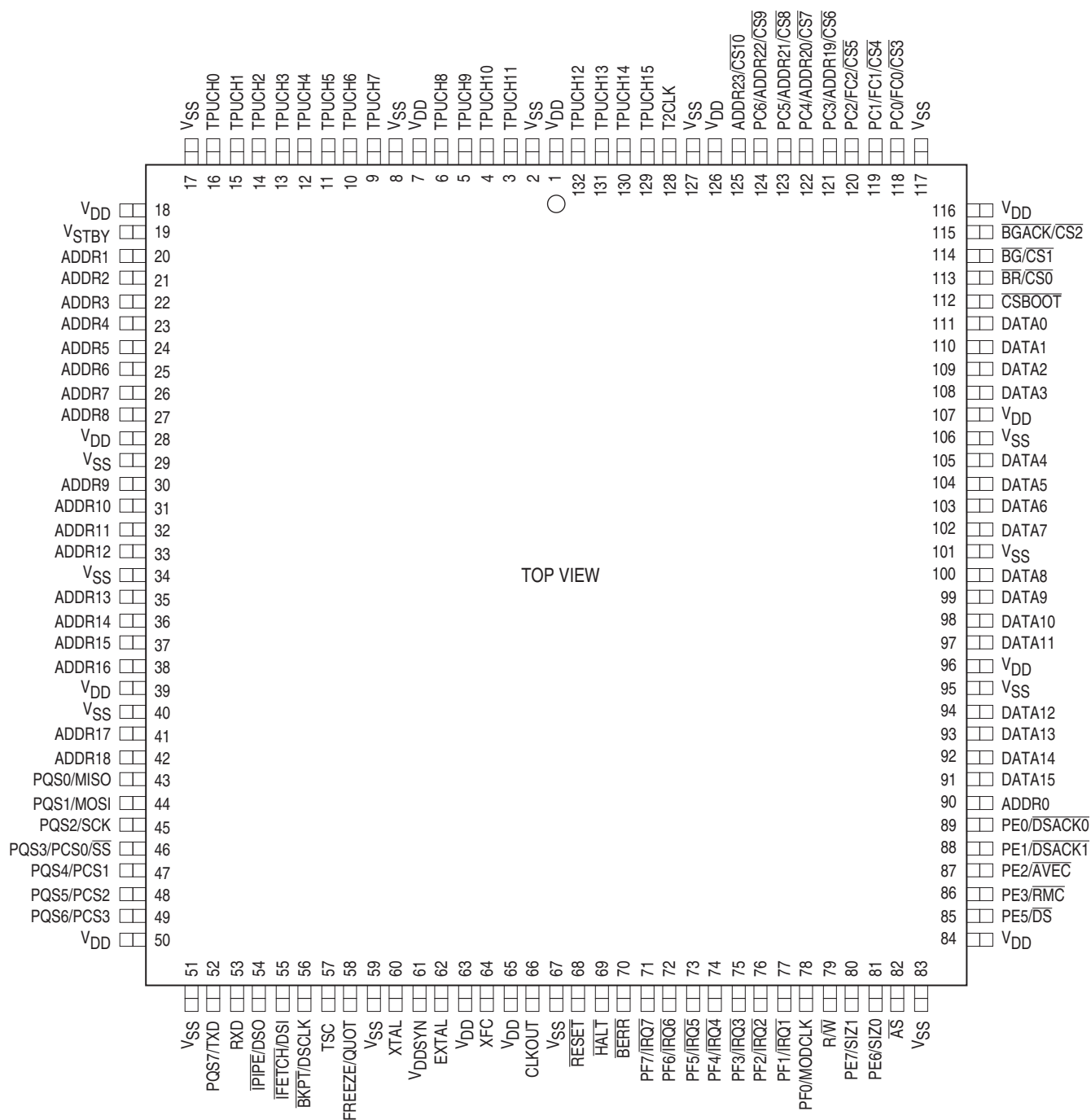
Figure 3. CERQUAD Terminal Designation
