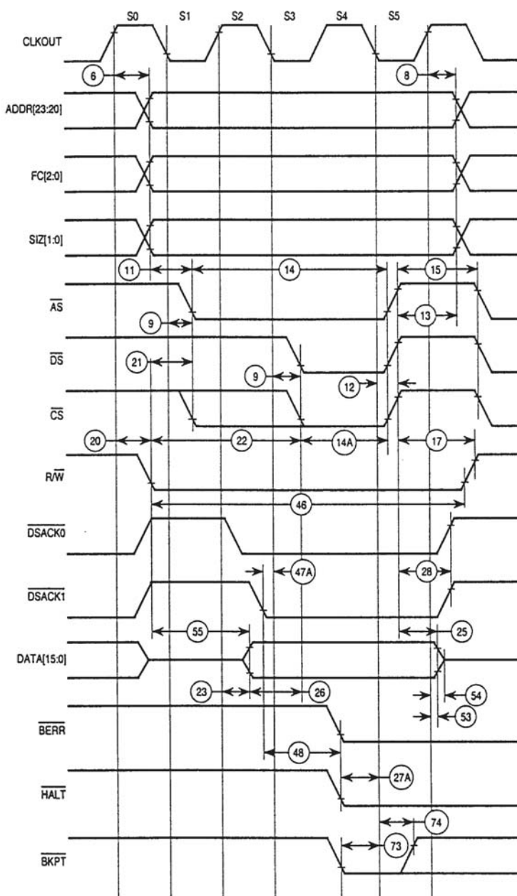
Figure 8. Write Cycle Timing Diagram
