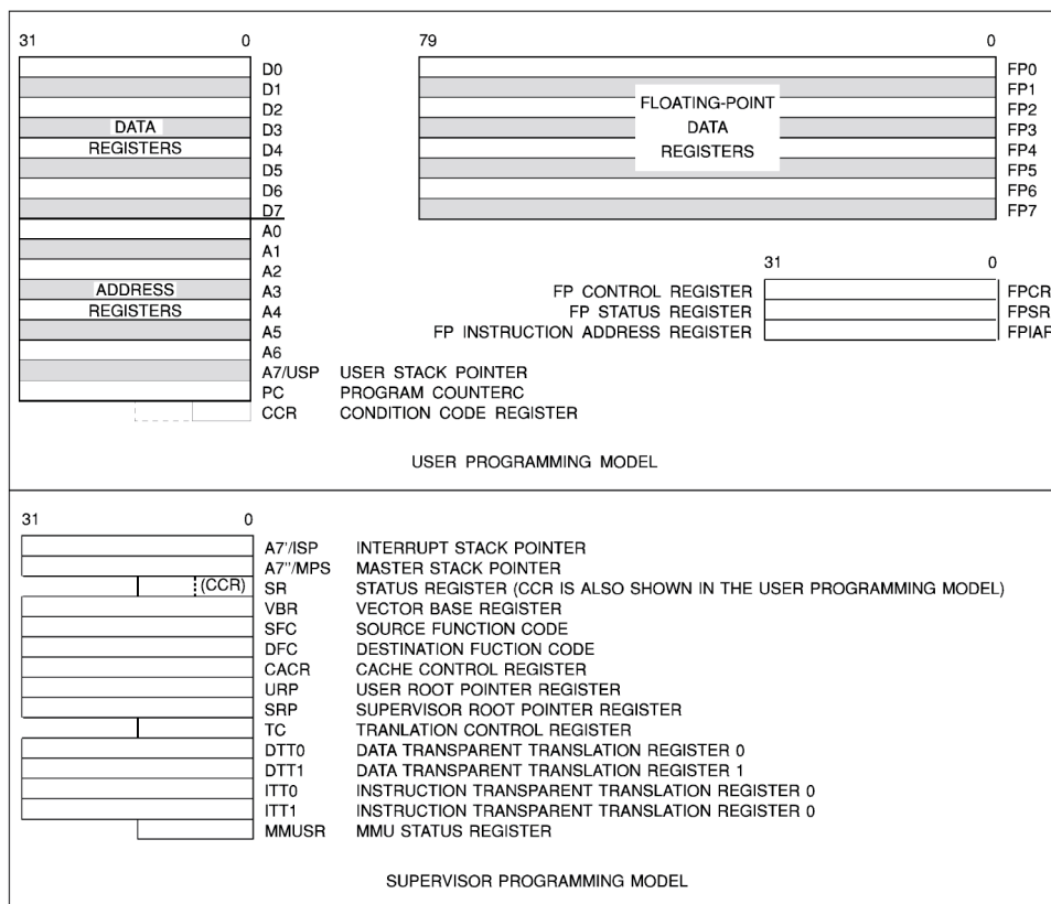
Figure 20. Programming Model
