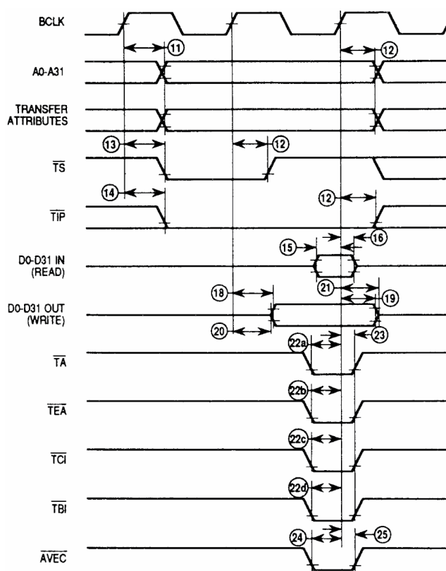
Figure 9. Read/Write Timing
