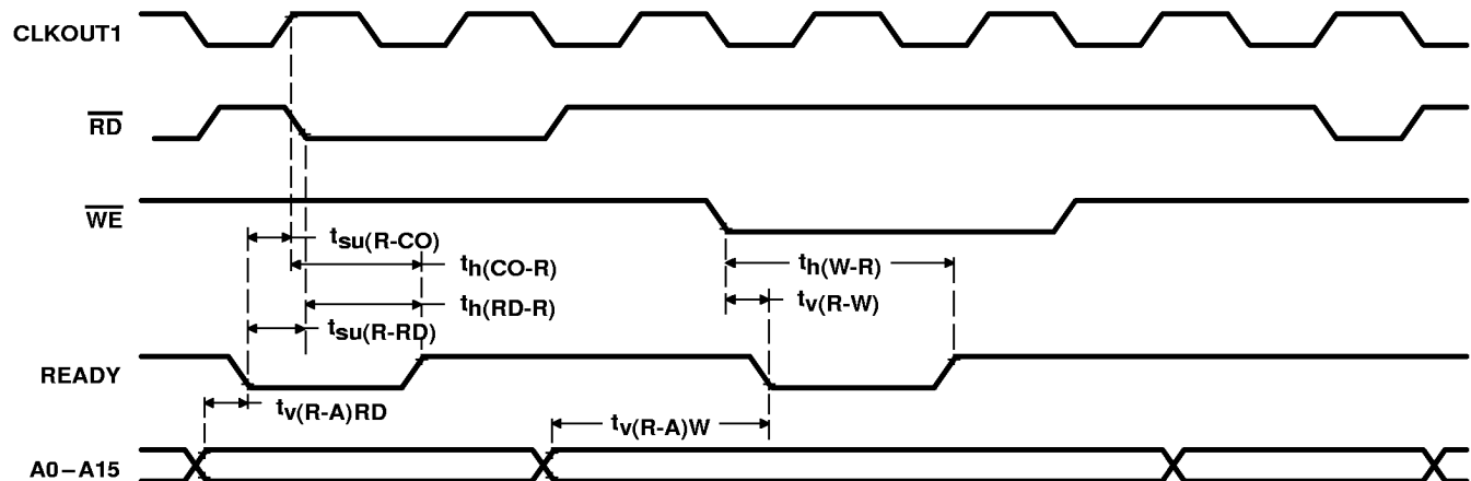
Figure 11. READY Timing
