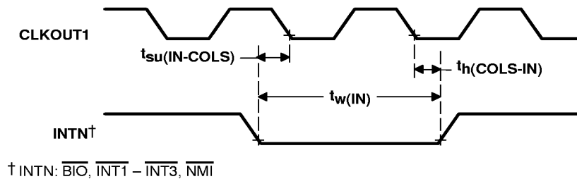
Figure 14. Interrupts and \overline{\text{BIO}} Timing
