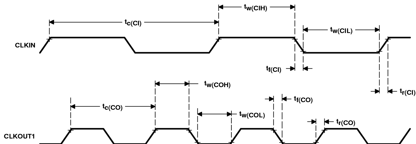
Figure 8. CLKIN-to-CLKOUT1 Timing With PLL (Enabled)
