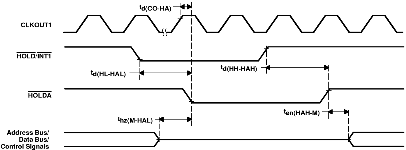
Figure 15. External DMA Timing
