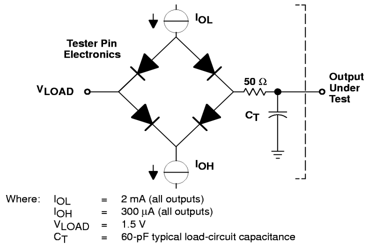
Figure 3. Test Load Circuit
