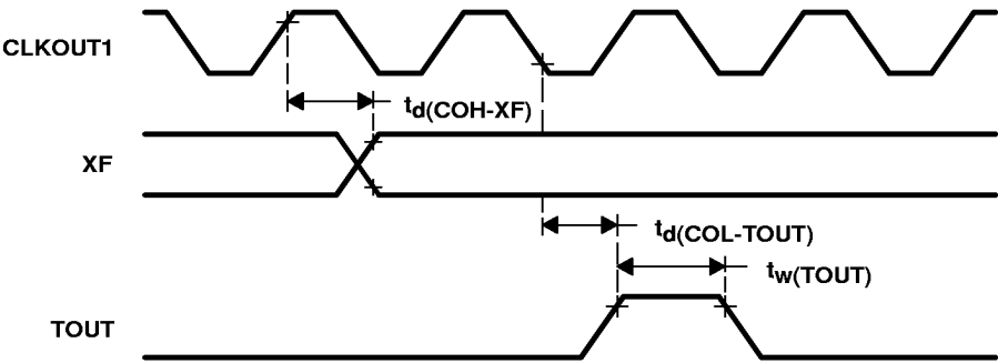
Figure 12. XF and TOUT Timing
