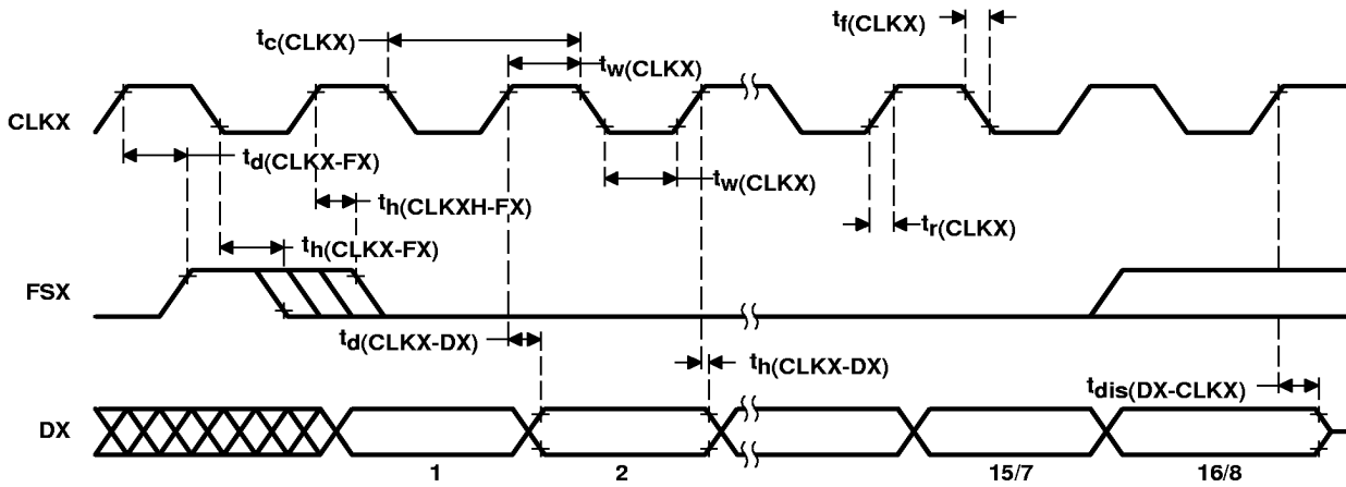
Figure 17. Serial-Port Transmit Timings
