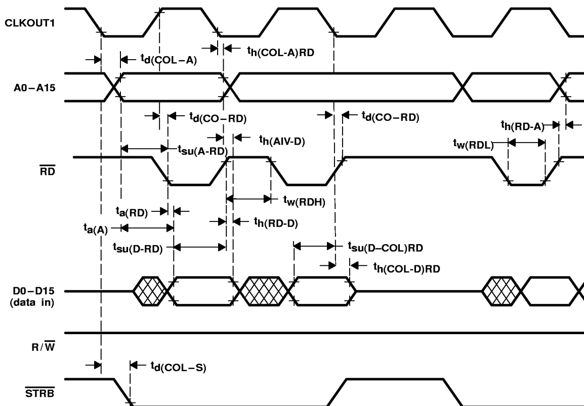
Figure 9. Memory Interface Read Timing
