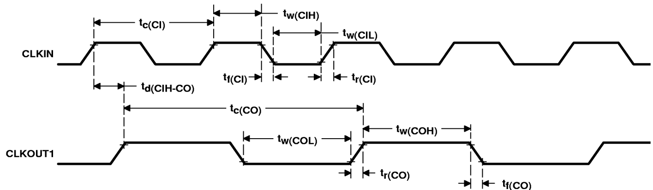
Figure 7. CLKIN-to-CLKOUT1 Timing Without PLL (using ÷2 clock option)
