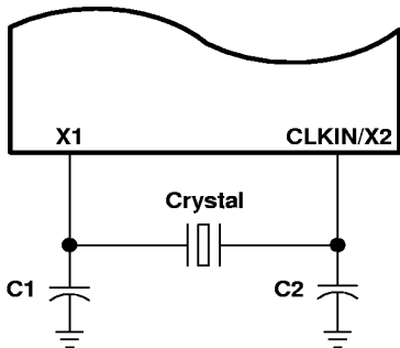
Figure 6. Internal Clock Option
