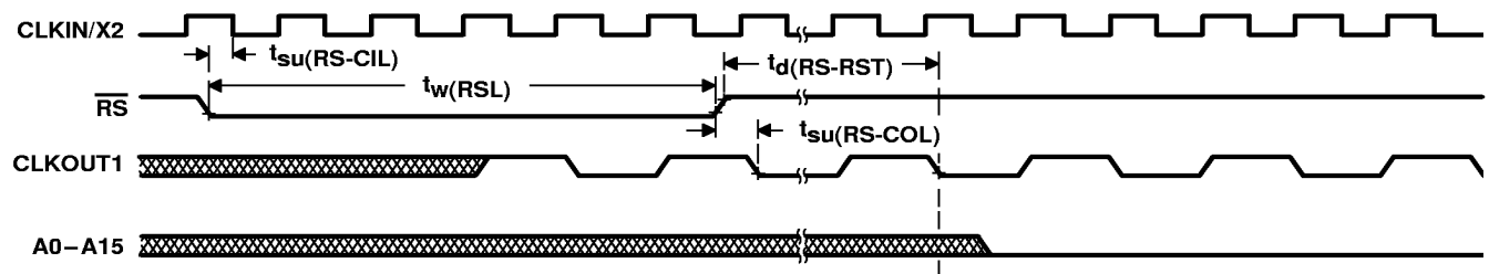
Figure 13. Reset Timing
