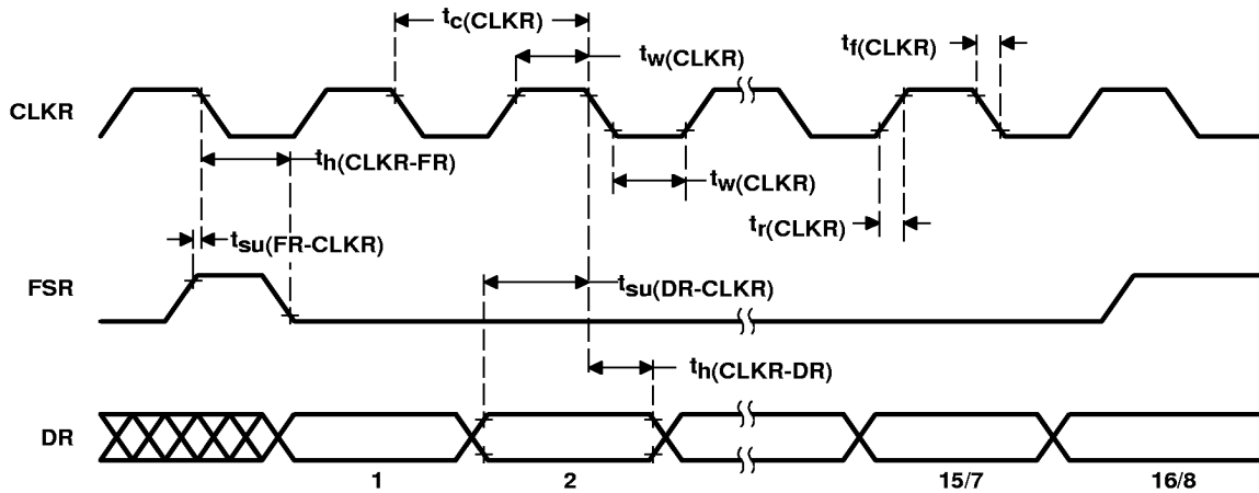
Figure 16. Serial-Port Receive Timing
