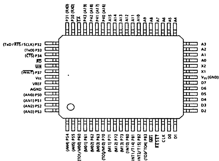
Figure 2.1 (2). Pin Assignment (Flat Package)
