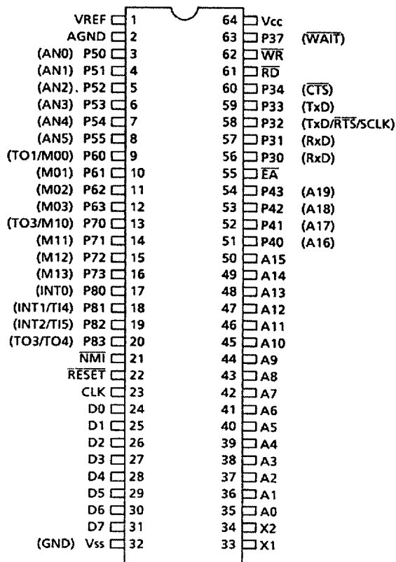
Figure 2.1 (1). Pin Assignment (Shrink Dual Inline Package)
