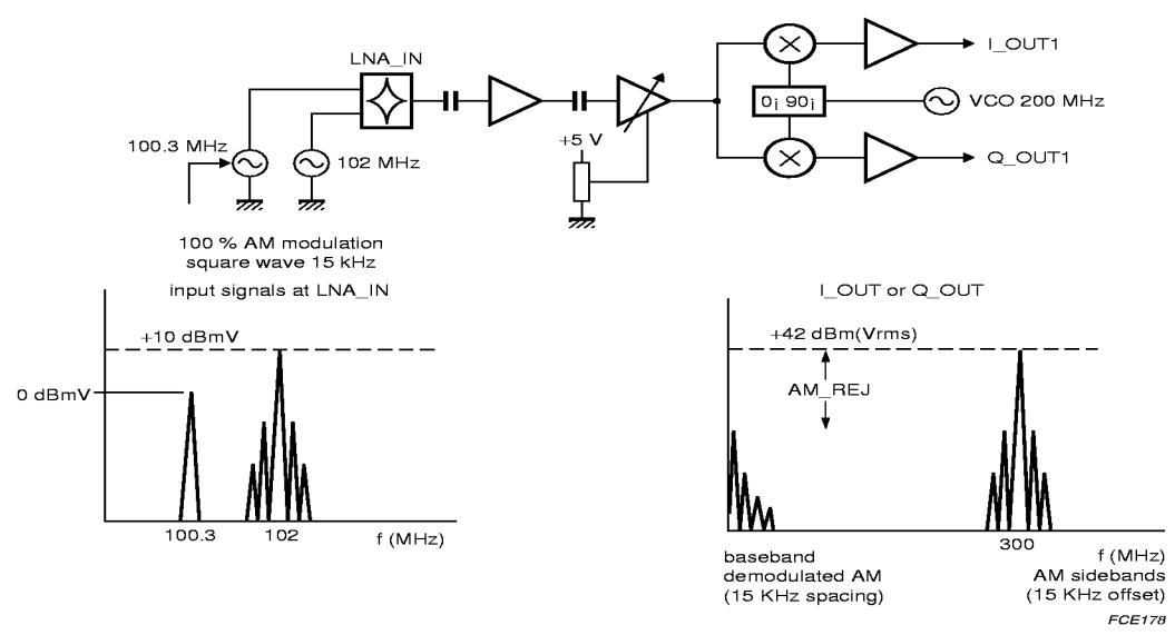
Fig.9 Overall AM rejection measurement.
