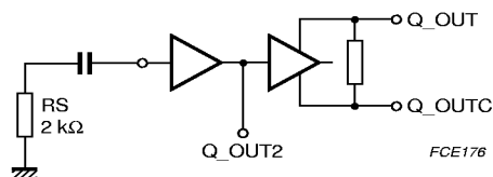
Fig.7 Noise measurement.
