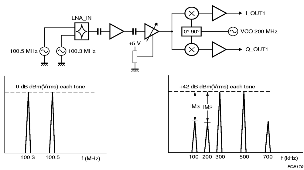
Fig.10 Overall IM3 measurement.
