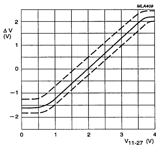
Fig.5 Difference between black level and measuring level at the RGB outputs ( \Delta V ) as a function of the brightness control input voltage ( V_{11} ).
