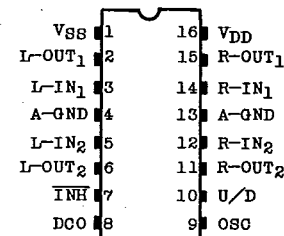
TC9153AP
