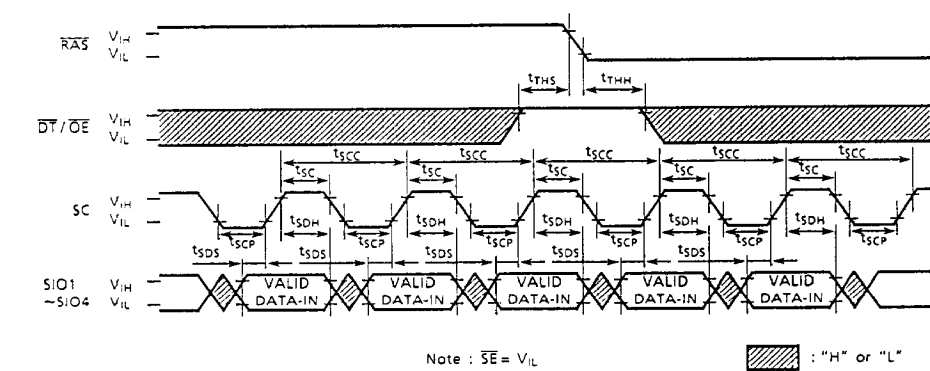
SERIAL WRITE CYCLE ( \overline{SE} = V_{IL} )
