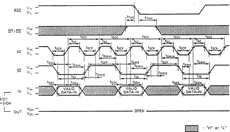
SERIAL WRITE CYCLE ( \overline{SE} Controlled Inputs)
