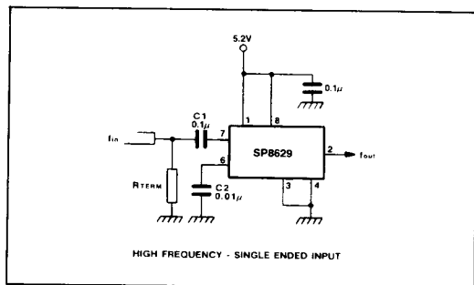
Fig.6 High frequency, single-ended input
