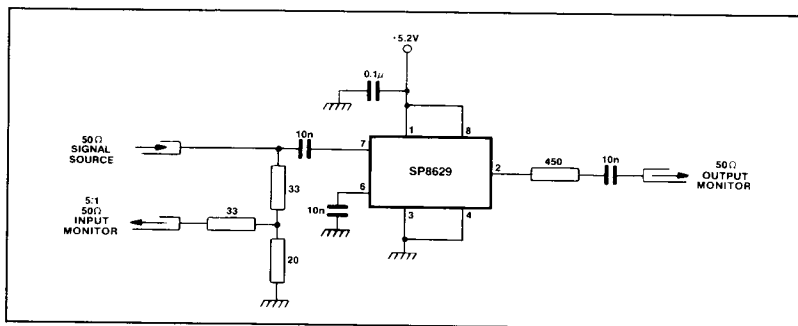
Fig.5 Test circuit
