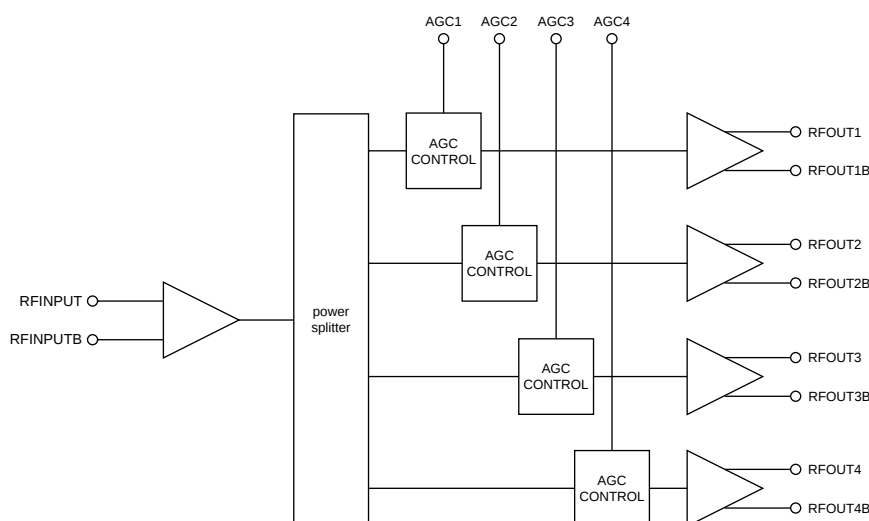
Figure 2 - SL2150F block diagram
