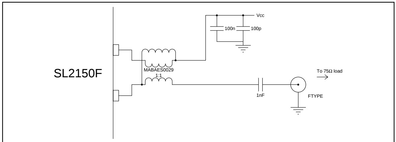
Figure 12 - Example application driving 75 \Omega load
