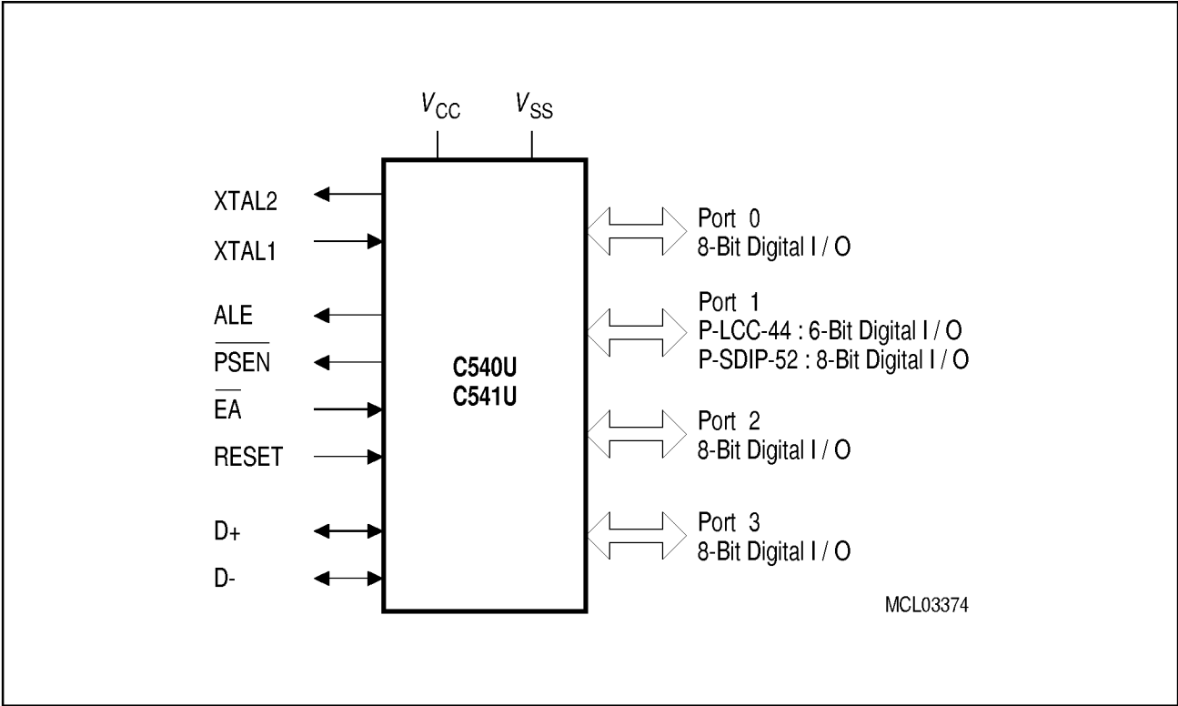
Figure 2 Logic Symbol
