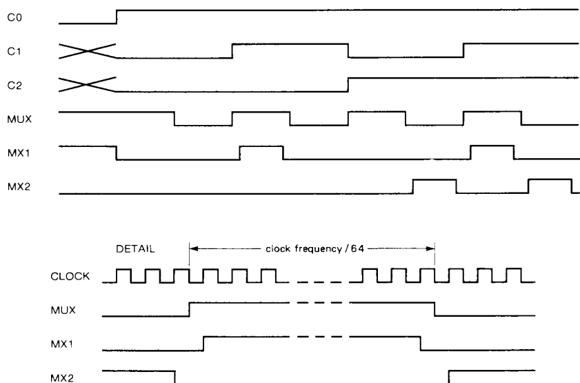
Fig. 4 Timing diagram.
