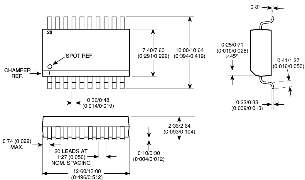
20-LEAD MINIATURE PLASTIC DIL - MP20
