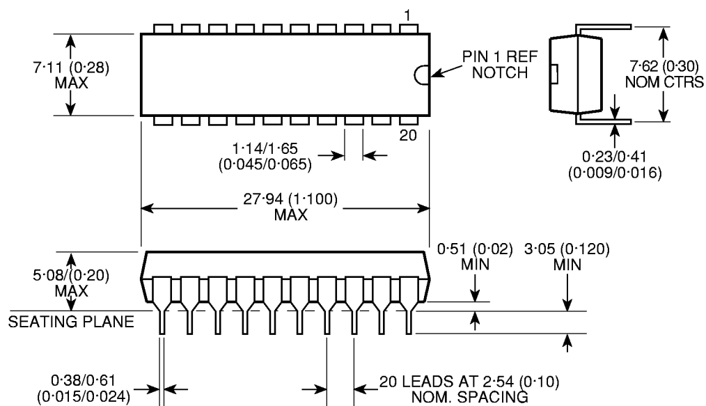
20-LEAD PLASTIC DIL – DP20
