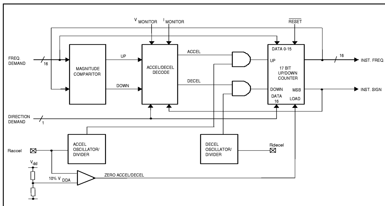
Fig. 4: Acceleration/deceleration block
