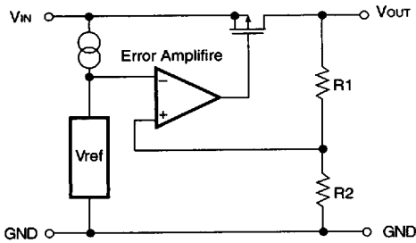
FIG. 1 Block Diagram
