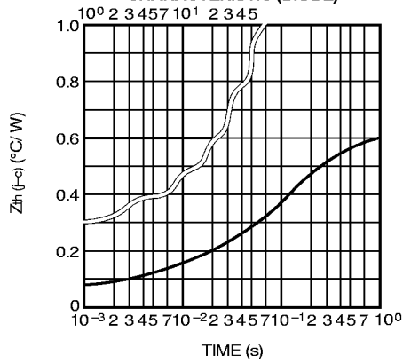
TRANSIENT THERMAL IMPEDANCE CHARACTERISTIC (DIODE)
