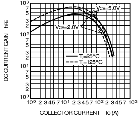
DC CURRENT GAIN VS. COLLECTOR CURRENT (TYPICAL)
