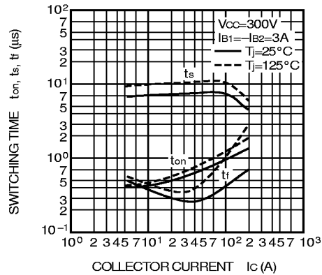
SWITCHING TIME VS. COLLECTOR CURRENT (TYPICAL)
