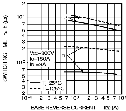
SWITCHING TIME VS. BASE CURRENT (TYPICAL)
