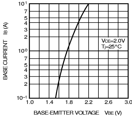
COMMON EMITTER INPUT CHARACTERISTIC (TYPICAL)
