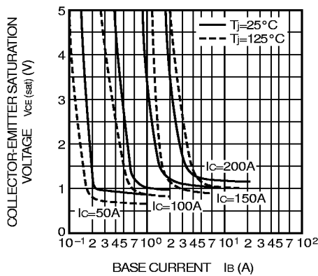
COLLECTOR-EMITTER SATURATION VOLTAGE (TYPICAL)
