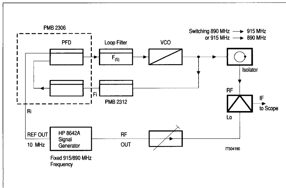
Figure 13 Measurement Set-Up for Lock-In Time
