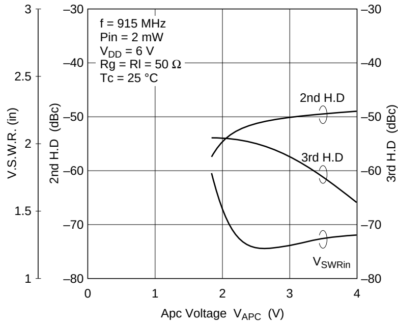
2nd H.D, 3rd H.D, VSWR (in) vs. V_{APC} (2)
