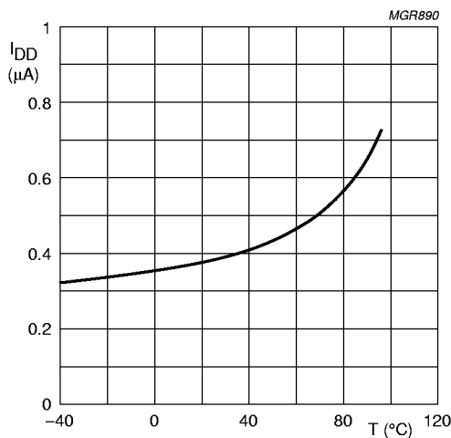
V_{DD} = 3 V; Timer = 1 minute.
