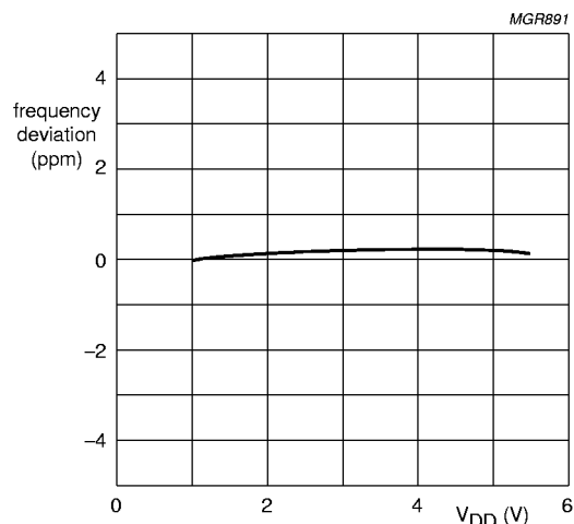
T_{amb} = 25 °C; normalized to V_{DD} = 3 V.
