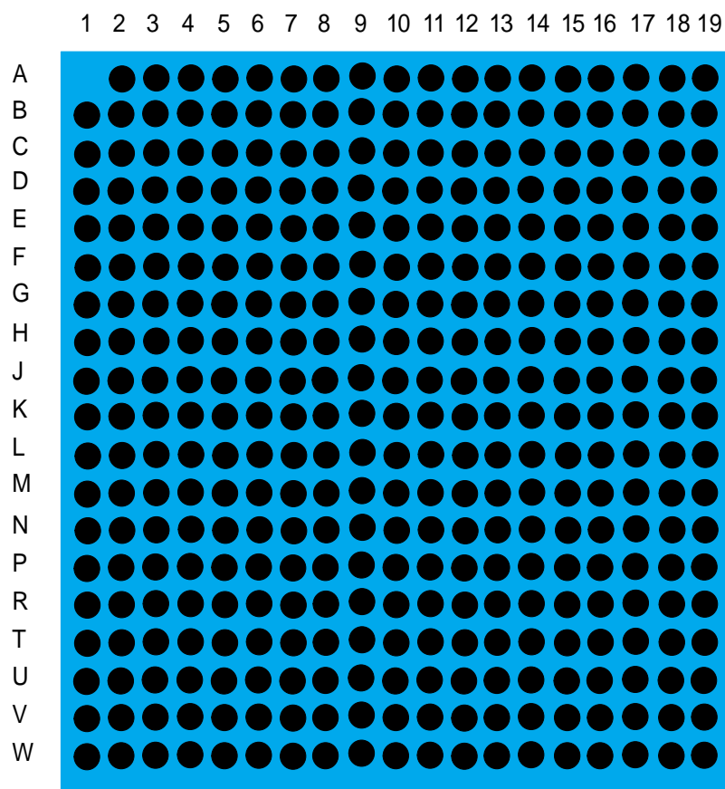
Figure 3. Pinout of the PC755B, 360 PBGA, CBGA and CI-CGA Packages as Viewed from the Top Surface
