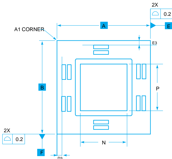
Figure 28. Mechanical Dimensions and Bottom Surface Nomenclature of PC755B (CI-CGA)
