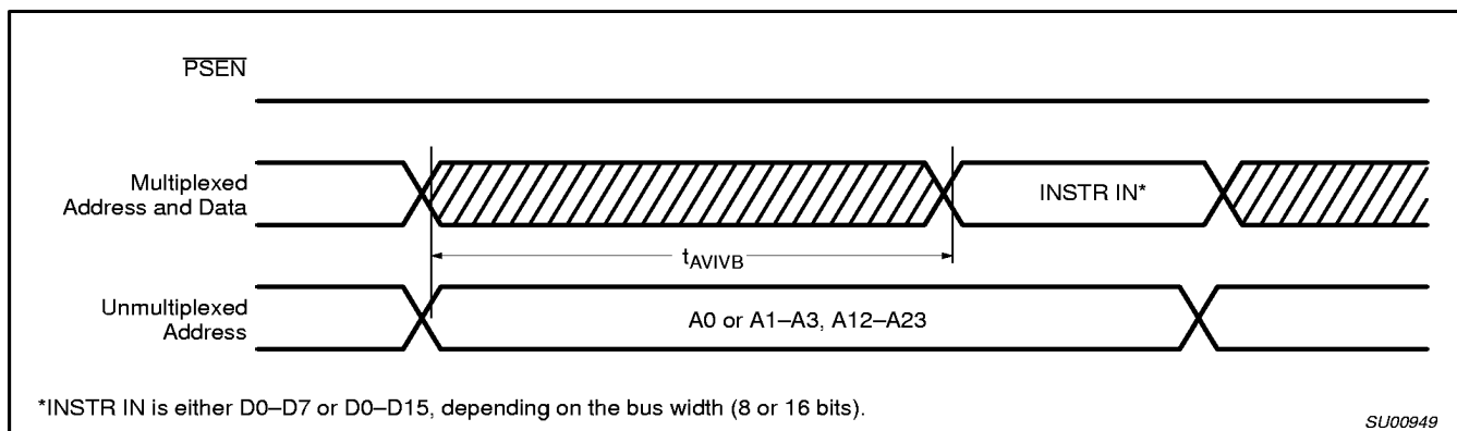
Figure 9. External Program Memory Read Cycle (Non-ALE Cycle)
