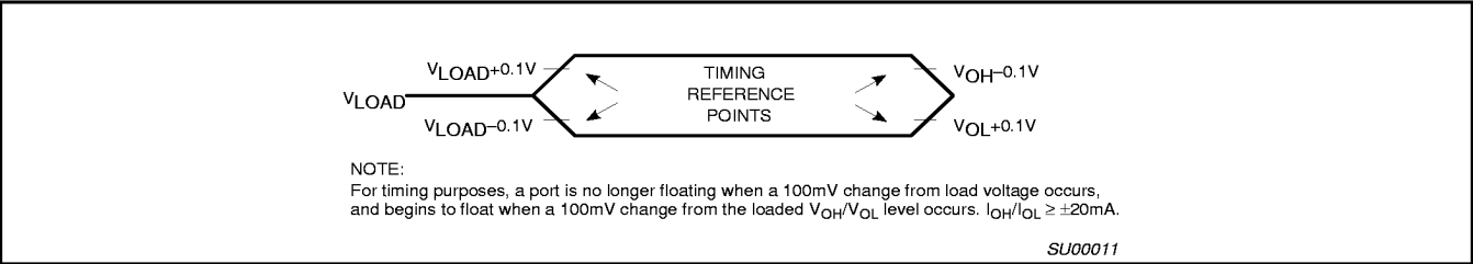
Figure 16. Float Waveform
