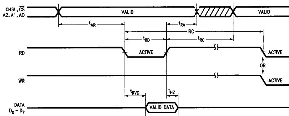
Read Cycle
