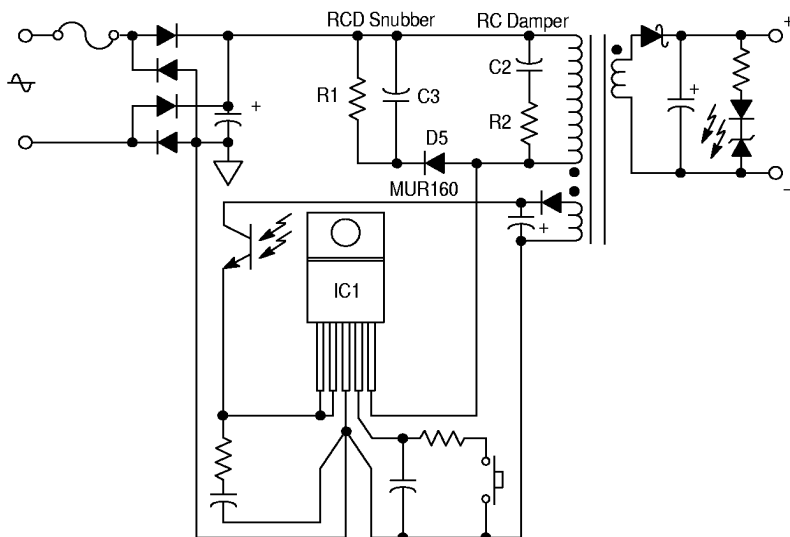
Figure 29. Snubber and Damper Circuits
