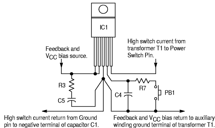
Figure 30. Recommended Printed Circuit Board Layout
