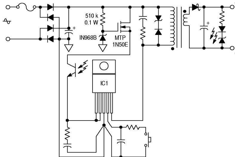
Figure 33. Transformer Auxiliary Winding Elimination MOSFET Transistor Series Regulator Method
