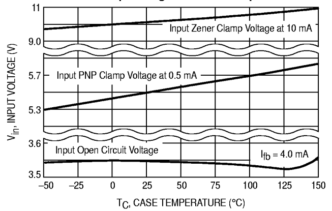
Figure 4. State Control Input Open Circuit and Clamp Voltages versus Temperature
