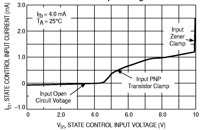
Figure 2. State Control Input Current versus Input Voltage
