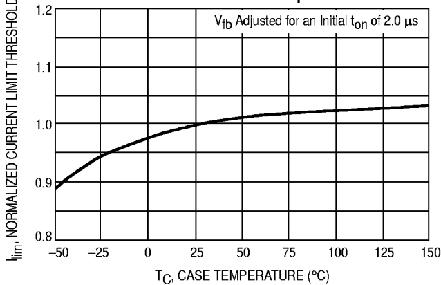
Figure 11. Power Switch Circuit Current Limit Threshold versus Temperature
