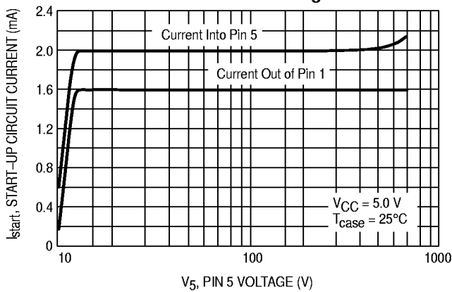
Figure 9. Start-Up Circuit Current versus Pin 5 Voltage
