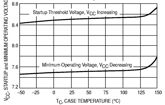
Figure 8. Undervoltage Lockout Thresholds versus Temperature
