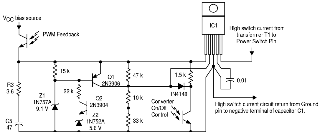
Figure 34. Converter Soft-Start
