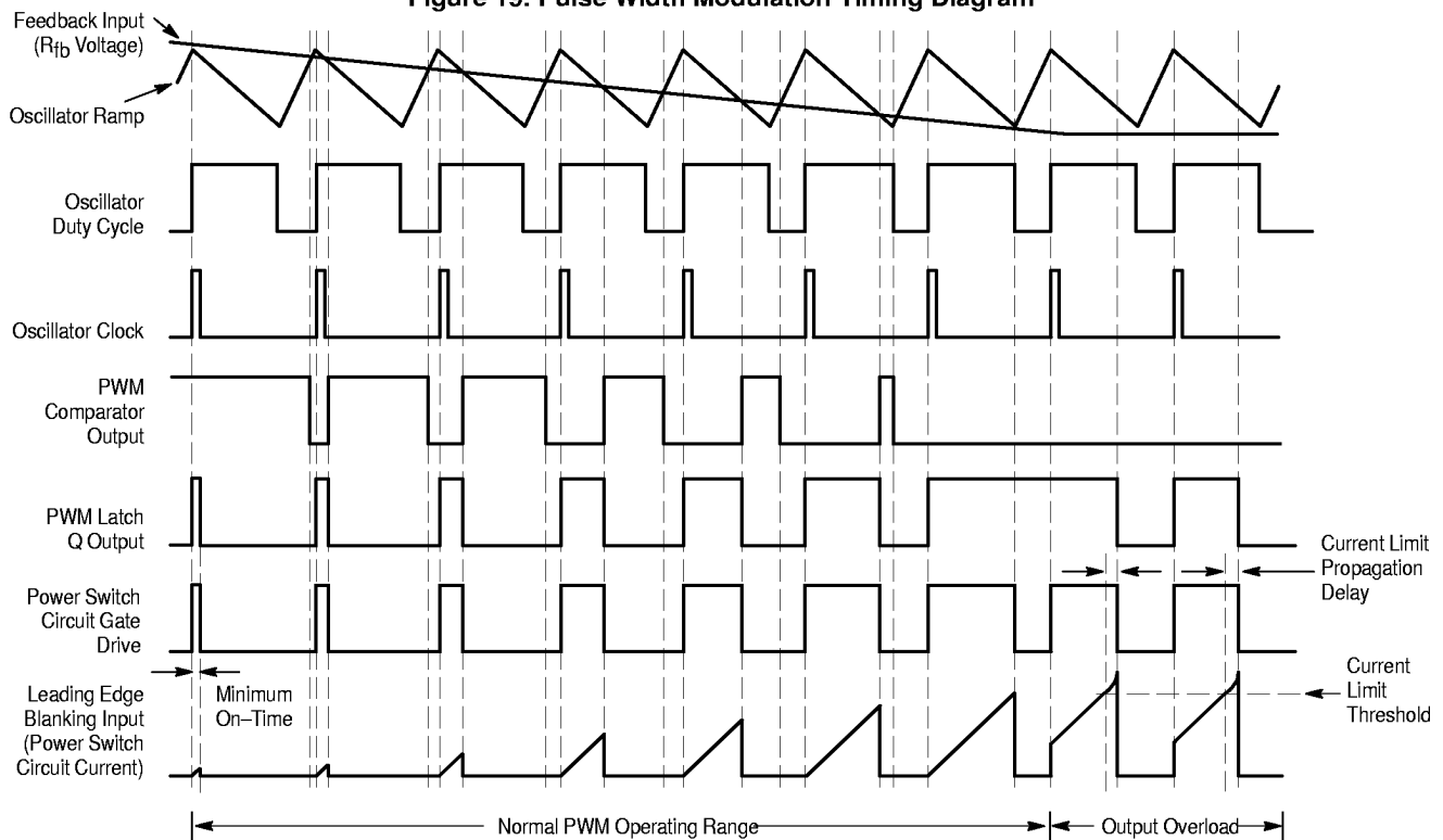
Figure 19. Pulse Width Modulation Timing Diagram
