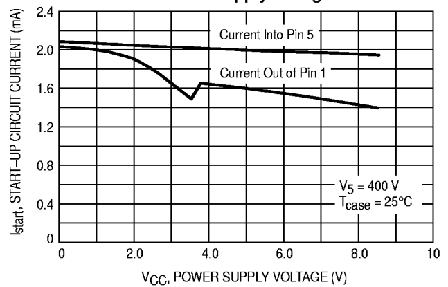
Figure 10. Start-Up Circuit Current versus Power Supply Voltage
