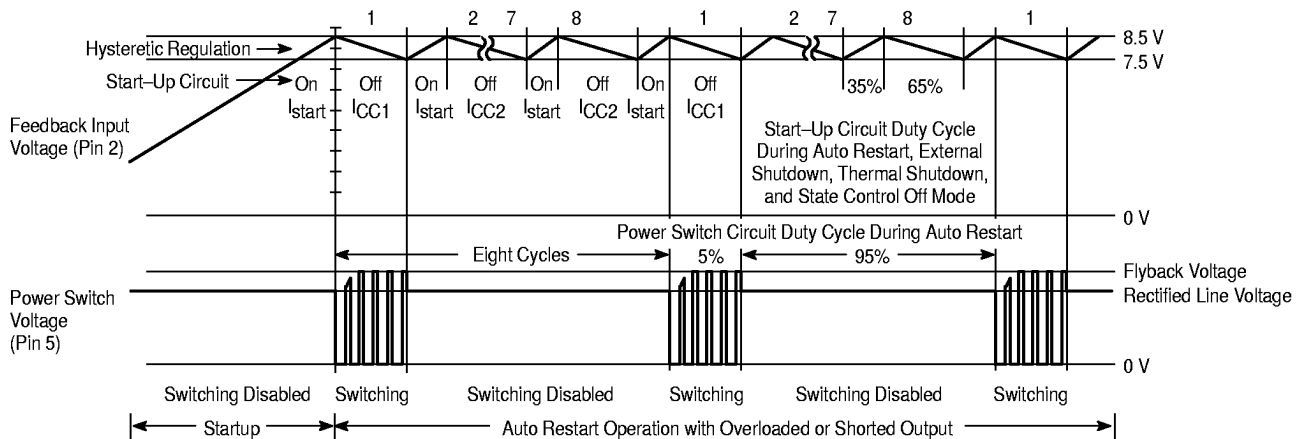
Figure 21. Auto Restart Operation Timing Diagram
