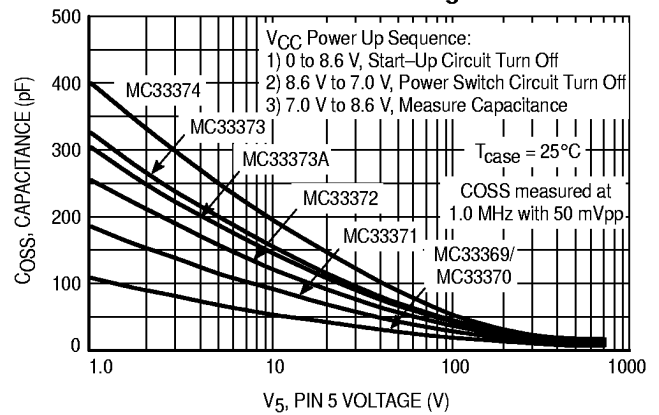
Figure 16. Power Switch Circuit Capacitance versus Pin 5 Voltage
