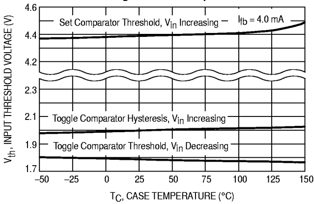
Figure 3. State Control Input Threshold Voltage versus Temperature
