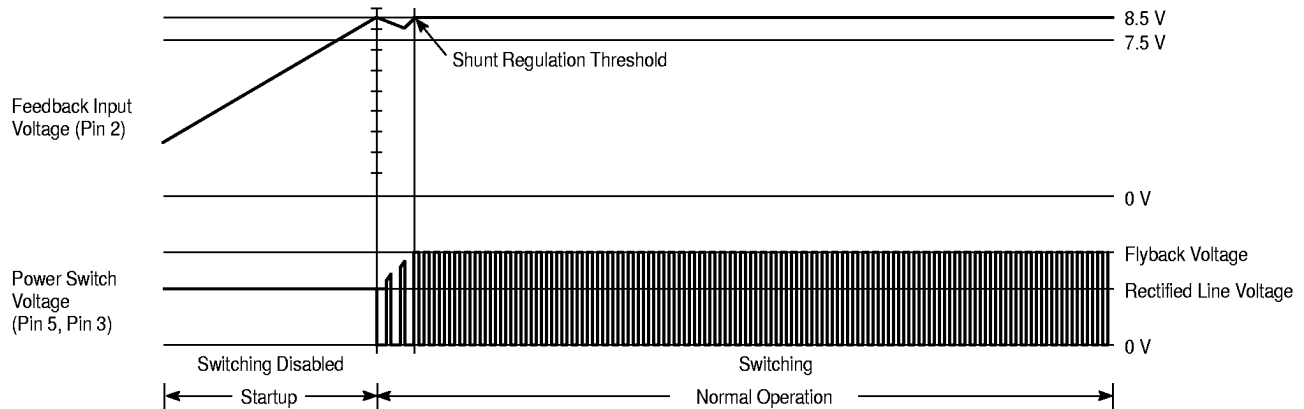
Figure 20. Startup and Normal Operation Timing Diagram
