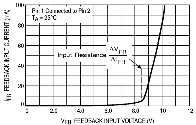
Figure 6. Feedback Input Current versus Input Voltage
