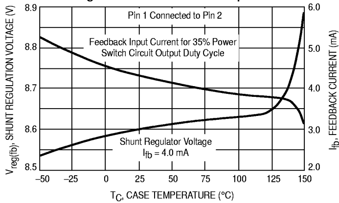
Figure 7. Feedback Input Shunt Regulation Voltage and Current versus Temperature
