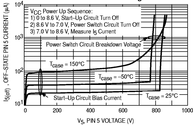
Figure 15. Power Switch Circuit Off-State Current versus Voltage
