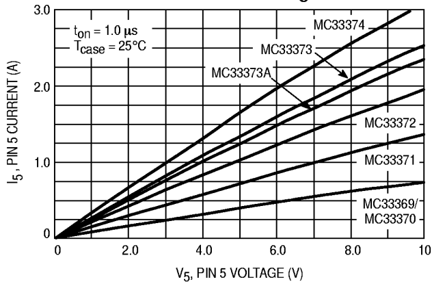
Figure 13. Power Switch Circuit Current versus Pin 5 Voltage
