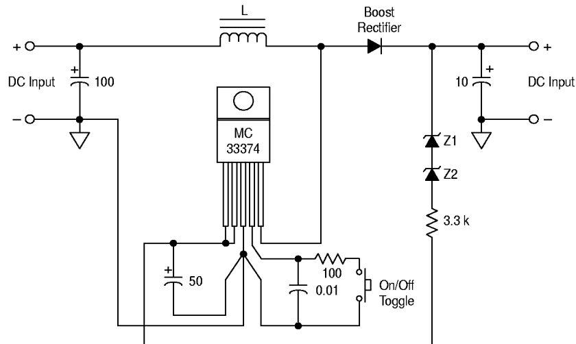
Figure 35. High Voltage Step-Up Converter
