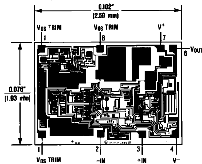
Chip Topography
